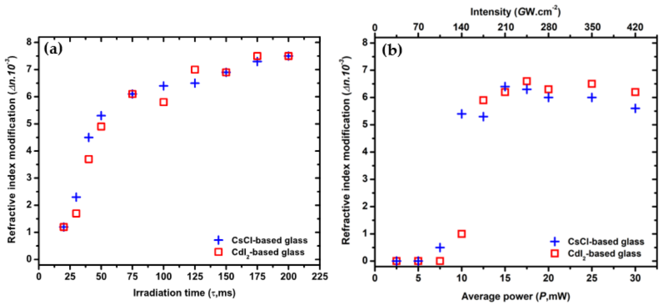
Figure 3. Evolution of the refractive index modification ( \Delta n ) as a function of (a) the irradiation time ( \tau ) at 20 mW and (b) the average power ( P ) and the corresponding intensity with \tau = 100 ms in the selected glasses for the step-index fiber (CsCl—(blue cross) and CdI 2 —(red square) based glasses).
