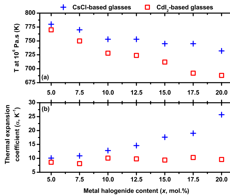
Figure 2. (a) Evolution of the measured temperature at a viscosity of 10 6 Pa·s as a function the metal halide CsCl (blue crosses) or CdI 2 (red squares) content. (b) Evolution of the thermal expansion coefficient as a function the metal halide CsCl (blue crosses) or CdI 2 (red squares) content.
