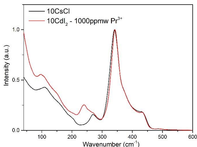
Figure 4. Raman spectra of the glasses ([\text{GeS}_2]_{0.80}\text{-}[\text{Ga}_2\text{S}_3]_{0.20})_{90}\text{-(CsCl)}_{10} and ([\text{GeS}_2]_{0.80}\text{-}[\text{Ga}_2\text{S}_3]_{0.20})_{90}\text{-(CdI}_2)_{10}\text{:1000 ppmw Pr}^{3+} recorded at 785\text{ nm} .
