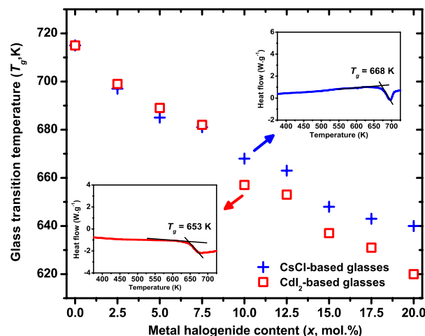
Figure 1. Evolution of T_g as a function the metal halide CsCl (blue crosses) or CdI 2 (red squares) content. Inset correspond to the DSC traces of glasses with 10 mol. % of CsCl (blue line) or CdI 2 (red line).
