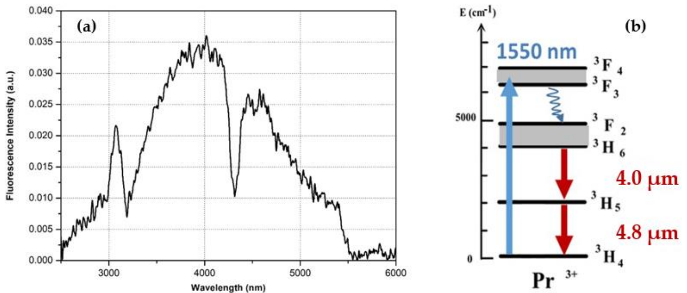
Figure 5. (a) Fluorescence intensity of the core of the double index fiber glasses ([GeS 2 ] 0.80 -[Ga 2 S 3 ] 0.20 ) 90 -(CsCl) 10 and ([GeS 2 ] 0.80 -[Ga 2 S 3 ] 0.20 ) 90 -(CdI 2 ) 10 :1000 ppmw Pr 3+ as a function of the wavelength; (b) energy level diagram of ion Pr 3+ .
