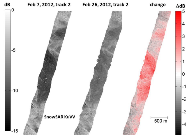
Figure 10. Demonstration of observed Ku-band VV-pol backscattering from two consecutive SnowSAR flight campaigns in Sodankylä, Finland. The difference in backscatter is depicted on the right, with red implying an increase. Increases in measured backscattering are correlated with the increase in SWE. The measured SWE between the flights increased on average by 41 mm in non-vegetated areas, which show the highest increase (figure adapted from Lemmetyinen et al., 2014).
