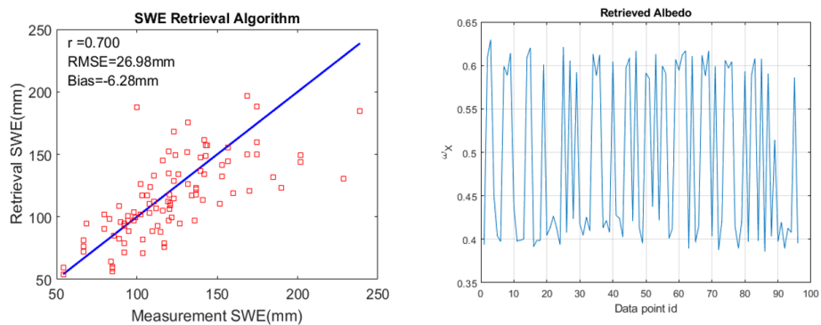
Figure 15. (a) SWE retrieval performance and (b) scattering albedo retrieval using Canadian SnowSAR 2013 X- and Ku-band radar data. The figures are from Zhu et al. (2018) and Zhu (2021).
