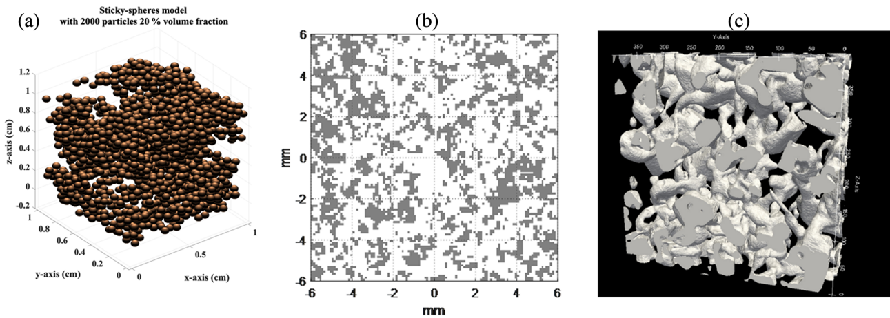
Figure 2. Microstructural descriptions of the snowpack: (a) sticky-hard-sphere theoretical model, (b) a bicontinuous medium with ice crystals in dark and air in white based on parameters (\zeta) = 1 mm and b = 1.0 , and (c) 3-D image from X-ray microtomography with ice crystals shown in white and air voids in black.
