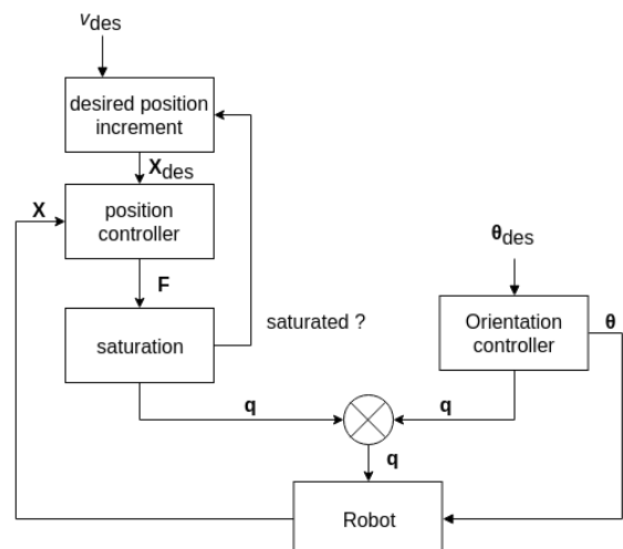
Fig. 3 Control scheme.
