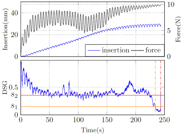
Fig. 4 Robot and DSG signals during an experiment
