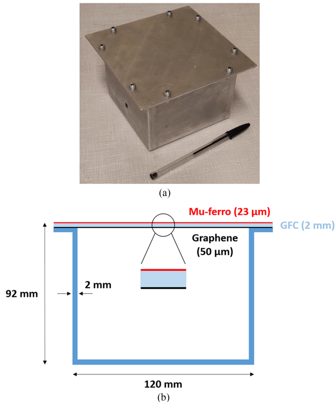
Fig. 1. (a) Al enclosure. (b) Schematic diagram with the trilayer composite cover.
