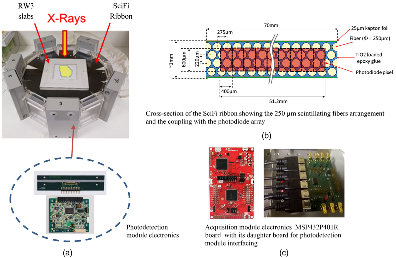
FIGURE 1 (a) Instrumented phantom prototype, (b) cross-section of the SciFi ribbons, and (c) signal acquisition electronics
