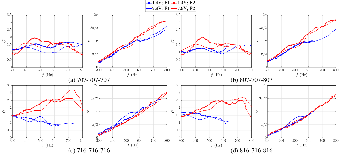
FIGURE 6: Gain G and phase \phi of the FDFs measured in TICCA-Spray showing comparison between the two operating points for the different swirler combinations (F1: blue, F2: red). Results are only plotted at two amplifier voltages V_0 = 1.4\text{ V} (solid line with marker) and 2.9\text{ V} (solid line without marker) to illustrate the differences.
