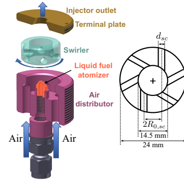
FIGURE 2: The injector unit comprises an air distributor, a hollow cone atomizer, a swirler, and a terminal plate. The terminal plate features a converging conical shape having a diameter of 8 mm at the outlet. The schematic of the swirler is shown on the right. The channel diameter d_{sc} and radial location R_{0,sc} can be changed to vary the swirl number and pressure drop.
