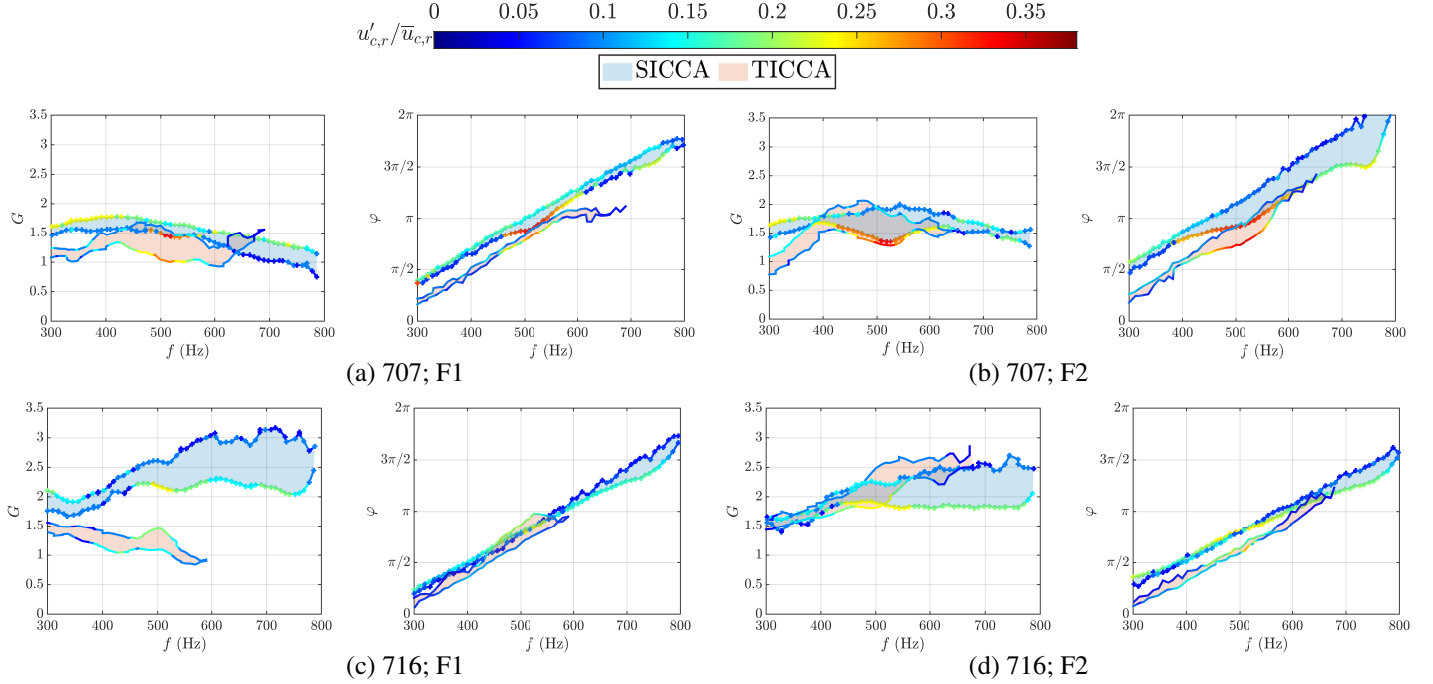
FIGURE 8: Comparison of gain G and phase \phi of the FDFs measured in the multiple-injector setup TICCA-Spray (solid lines without marker) with co-rotating neighbors and in the single-injector system SICCA-Spray (solid lines with marker) at the two operating points F1 and F2, and for the swirlers 707 and 716. The levels of velocity fluctuations u'_{c,r}/\bar{u}_{c,r} are indicated by the color levels and the span of the FDF data is represented by the colored bands.
