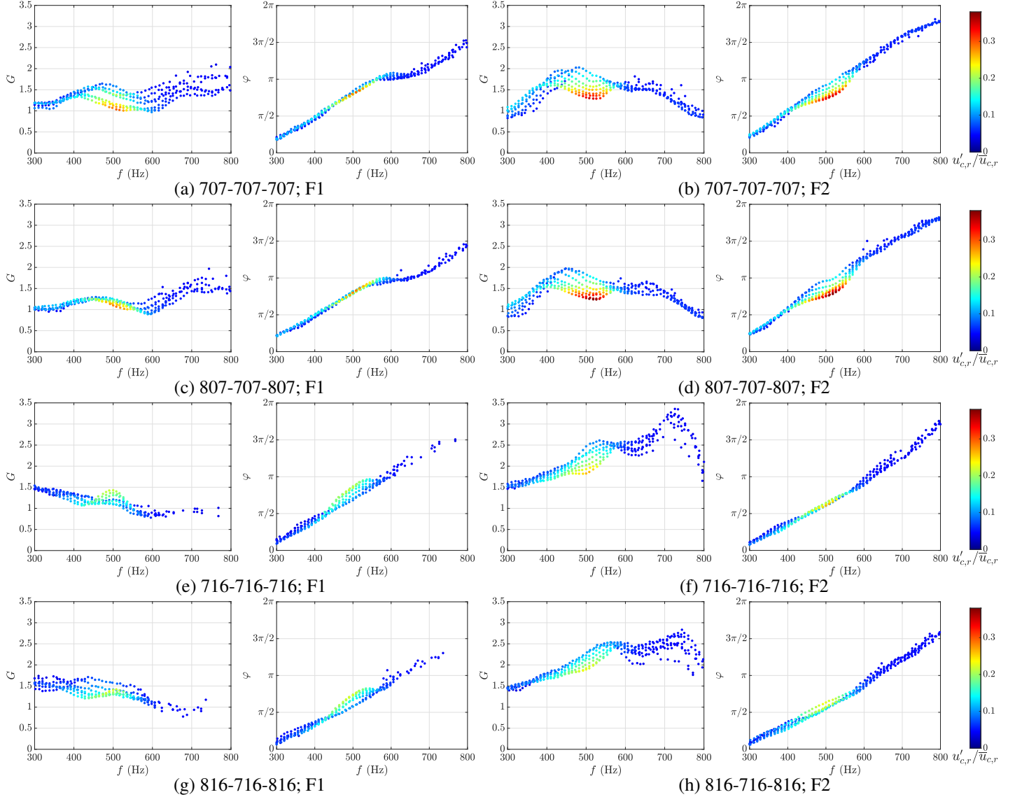
FIGURE 5: Gain G and phase \varphi of FDFs measured in TICCA-Spray at the two operating conditions. The color scale represent the velocity fluctuation levels measured at the injector outlet.
