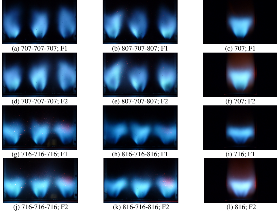
FIGURE 4: Flame images in TICCA-Spray (left and middle) and SICCA-Spray (right). Images are adjusted to have the same aspect ratio.
