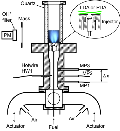
FIGURE 3: Sectional view of the TICCA-Spray combustor in a plane perpendicular to the length and passing through the central burner axis.
