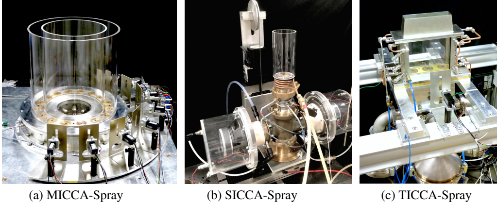
FIGURE 1: (a) Photograph of the MICCA-Spray test rig. The chamber mean diameter is 350 mm and the walls are 400 mm long. (b) View of the SICCA-Spray test rig. The cylindrical flame tube has a 69 mm inner diameter and is 200 mm long. (c) The linear combustor, namely TICCA-Spray, equipped with three injectors. Acoustic actuators are visible at the bottom of the photograph. A photomultiplier (in black) is installed in front of the window, behind a mask with a vertical rectangular slot serving as a spatial filter.
