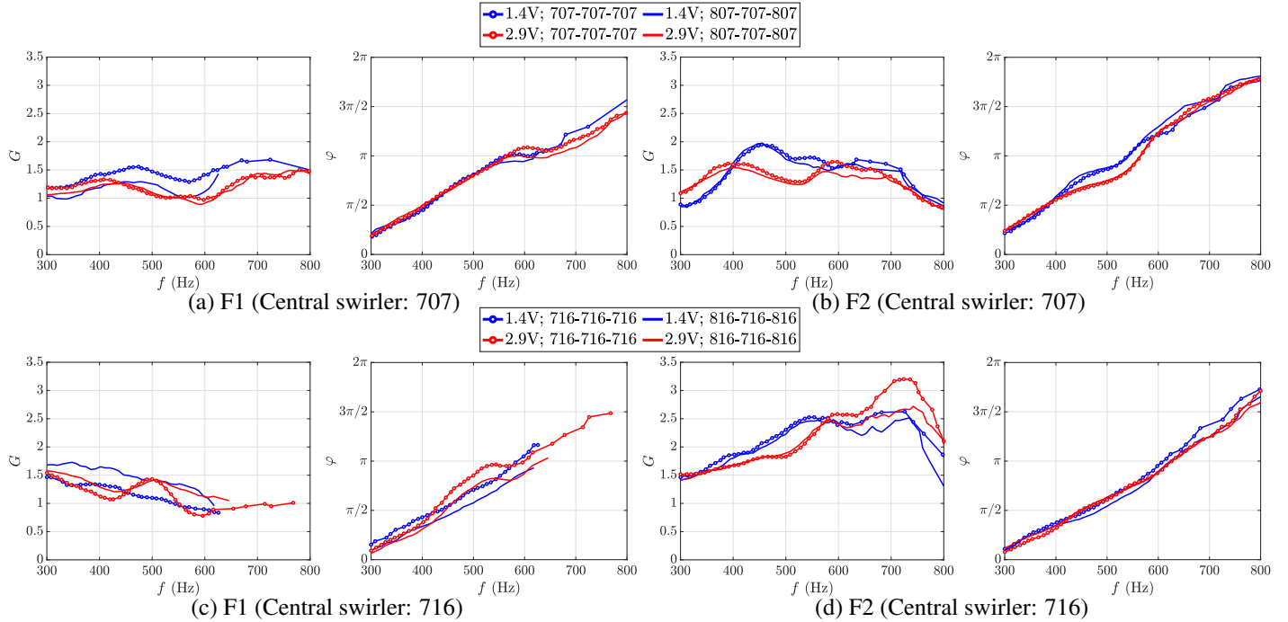
FIGURE 7: Gain G and phase \varphi of the FDF measured in TICCA-Spray with co- (solid lines with marker) and counter-swirl (solid lines without marker) swirler combinations at the two operating points F1 and F2. Results are presented for two amplifier voltage V_0 = 1.4\text{ V} and 2.9\text{ V} of the driver units.
