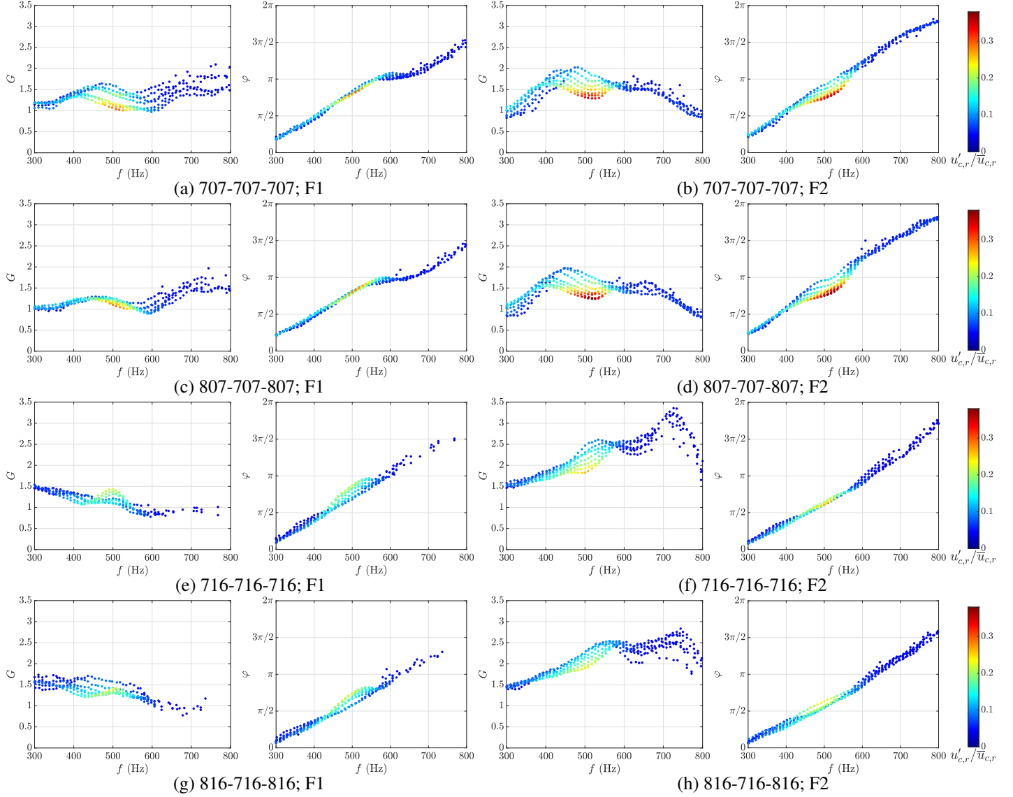
FIGURE 5: Gain G and phase \phi of FDFs measured in TICCA-Spray at the two operating conditions. The color scale represent the velocity fluctuation levels measured at the injector outlet.
