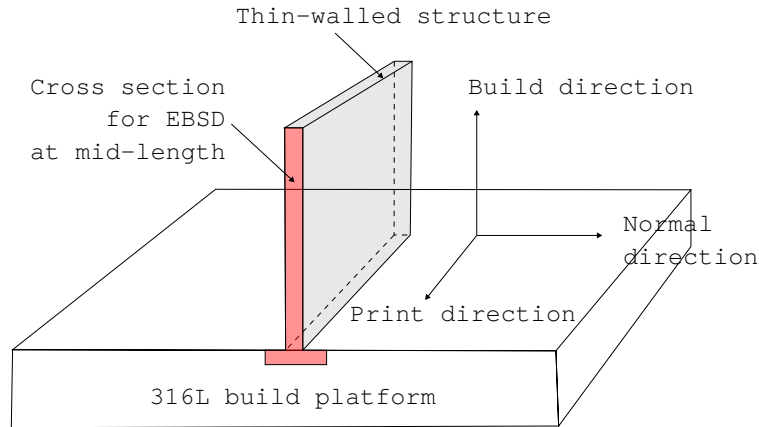
Figure 3: Illustration of the section of the wall, with the EBSD map area highlighted in red.
