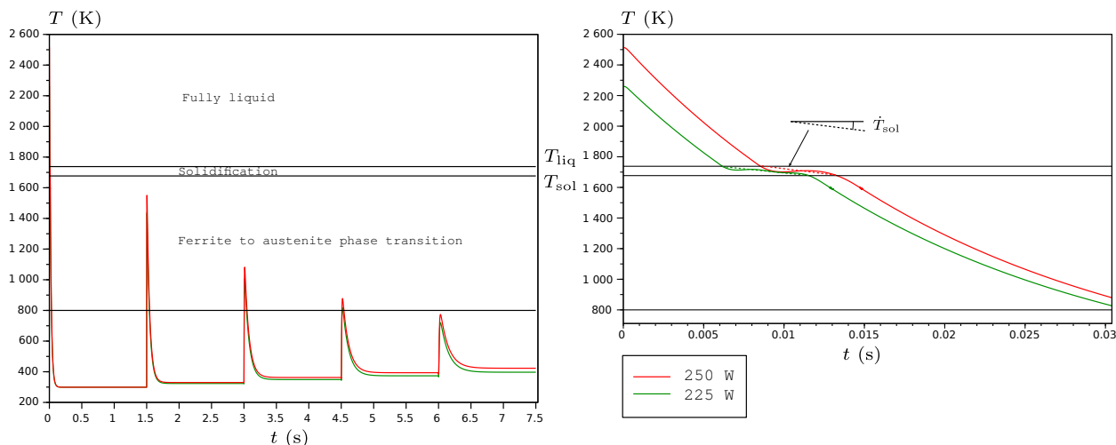
Figure 10: Computed temperature cycles (left) and magnification (right) (1st layer, 250 W and 225 W).
