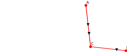
Fig. 4. Illustration of the SMOTE data augmentation technique. The red dots are the batch samples, and the black triangles are the synthetic new samples.
