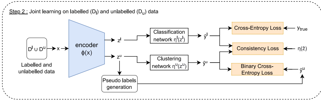
Fig. 2. Architecture of the joint learning step.
