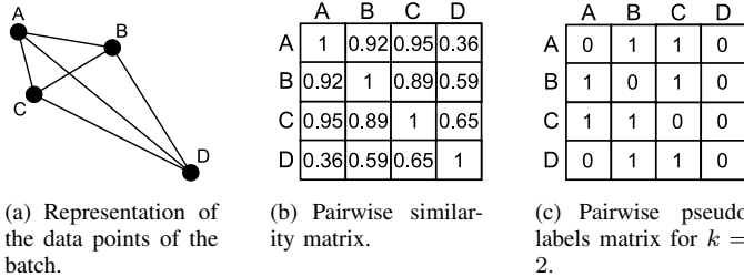
Fig. 3. The pairwise pseudo labels definition process with the threshold \lambda .
