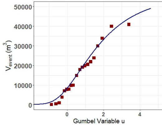
Fig. 2. Claret's Frequency - Magnitude curve obtained after the adjustment of recorded debris flow events using generalized Pareto distribution (Adapted from (?)).
