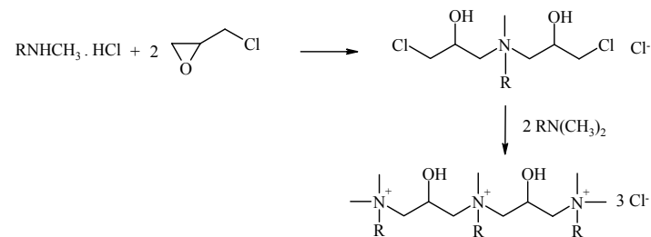
Scheme 6
