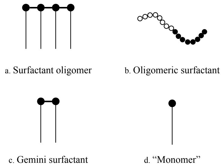
Figure 1 Surfactant oligomers (a), are distinguished from oligomeric surfactants (b) by the fact that the structural repeating unit is amphiphilic by itself. Surfactant oligomers are higher homologues of gemini surfactants (c). The structural repeating unit (d) corresponds to a conventional surfactant, which will be referred to as the “monomer”.
