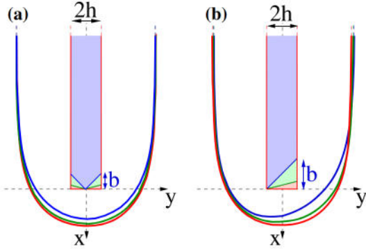
Fig. 6 Examples of cross sections ( \Gamma ) of the solid-liquid interface for blades of half-thickness h = 0.3\ell , with a tangential to normal velocity ratio \zeta = 0.1 , and various depths b of the wedge or the bevel. a Symmetric blades with b = 0 , b = 0.25\ell and b = \ell . b Asymmetric blades with b = 0 (red), b = 0.5\ell (green) and b = 2\ell (blue). Note that these values of b have been chosen so that the angle formed by the inclined face of the blades with axis y are the same from (a) to (b)
