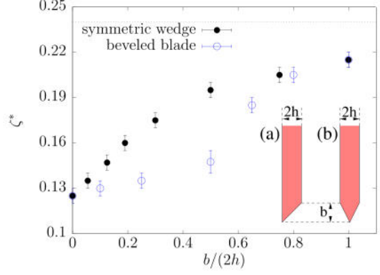
Fig. 7 Critical normal to tangential velocity ratio, \zeta^* , as a function of b/(2h) , for blades of thickness 2h = 0.6\ell , with a symmetric wedge at the cutting edge (black disks) and with a bevelled (blue circles). Dashed line indicates the value of \zeta^* found for blades modelled as a half plane. Inset: reminder of the shape of the cross section of a blade with a terminal symmetric wedge (a) , and a bevelled blade (b)
