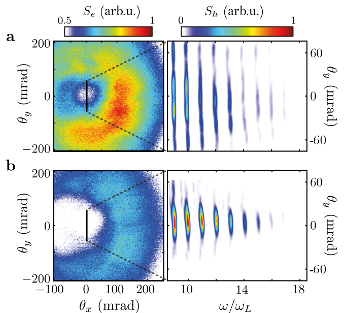
FIG. 3. Two-color ( \omega_L + 2\omega_L ) driver: Angular emission pattern of accelerated electrons (left) and angularly-resolved harmonic spectrum (right) obtained with a gradient scale length L_g \lesssim \lambda_L/50 and for phase delays maximizing either the electron emission \tau_{\phi,e} , (a), or the high-order harmonic emission \tau_{\phi,h} (b). The vertical black lines in the electron beam profiles mark the XUV spectrometer angular acceptance.
