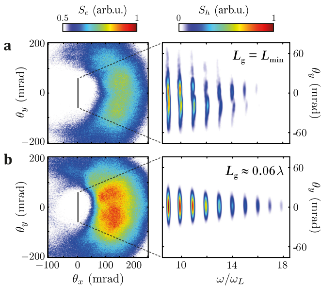
FIG. 2. Single-color ( \omega_L ) driver: Angular emission pattern of accelerated electrons (left) and angularly-resolved harmonic spectrum (right) obtained with the minimal gradient scale length L_g \lesssim \lambda_L/50 (a) and with a gradient scale length optimizing both ROM HHG and vacuum-laser-accelerated electron emission (b). The vertical black lines in the electron beam profiles mark the XUV spectrometer angular acceptance.
