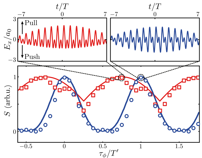
FIG. 5. Ejected electron charge (red squares) and high-order harmonic energy (blue circles) as function of the phase delay \tau_\phi , obtained from 2D PIC simulations. Full blue and red lines show the normalized heuristic model predictions S(\tau_\phi) and P(\tau_\phi) for E-field steepness ( n = 9 here) and maximum pulling E-field, respectively. The periodic modulations of these electronic and harmonic signals are shifted by \simeq T'/4 . The insets above show the driving fields for maximum electron (left) and high-harmonic (right) emission. A positive-valued electric field pulls electrons out of the plasma into vacuum.
