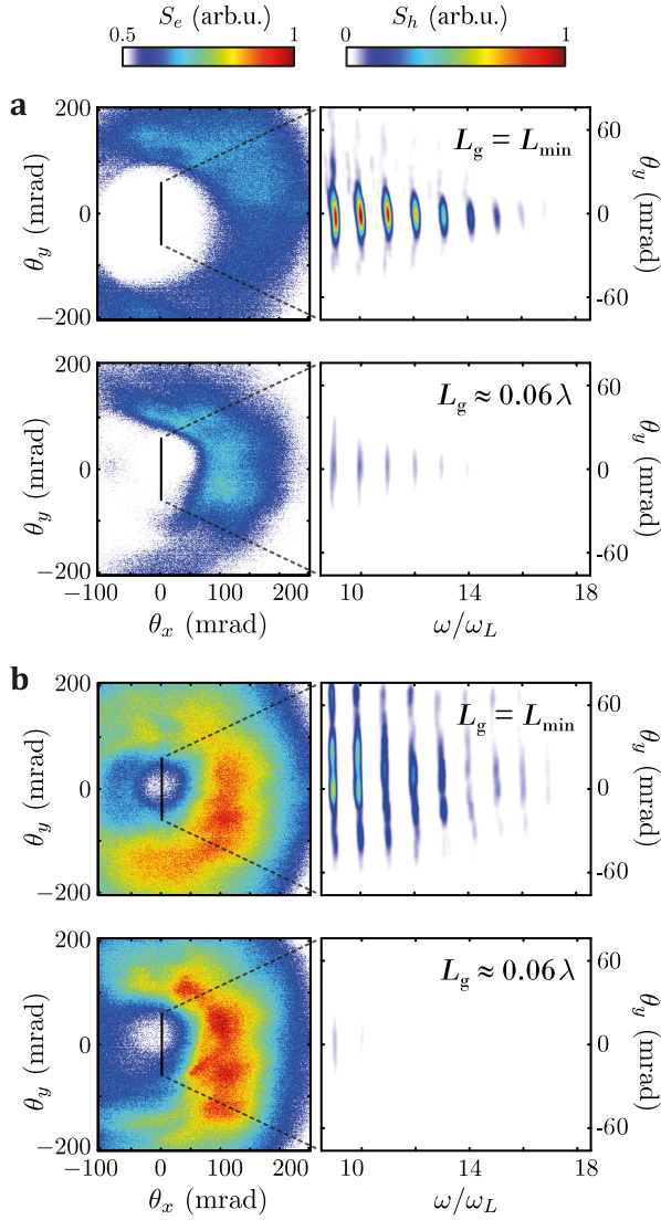
FIG. 8. Angular emission pattern of accelerated electrons (left) and angularly-resolved harmonic spectrum (right) obtained with the same two gradient scale lengths as in Fig.2 ( L_g \approx \lambda/50 above and L_g \approx \lambda/16 below). The phase delay of the two-color driving waveforms is set such that it optimizes low-divergence ROM HHG emission (a) or fast electron emission (b). The vertical black lines in the electron beam profiles mark the XUV spectrometer angular acceptance.
