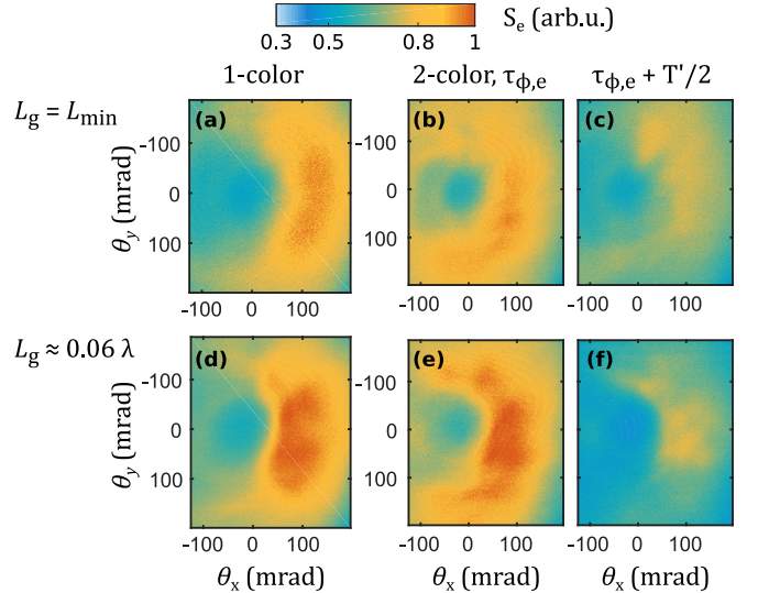
FIG. 10. Electron beam spatial profiles S_e measured with minimal plasma gradient scale length L_g \approx 0 (a)-(c) and with L_g \approx 0.06\lambda (d)-(f), and with a single-color ( \omega_L ) laser driver (a),(d), a two-color ( \omega_L + 2\omega_L ) driver with a phase delay \tau_\phi maximizing (b),(e) or minimizing (c),(f) the electron signal.
