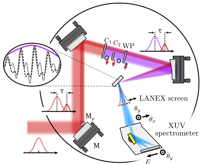
FIG. 1. (a) Experimental setup with the prepulse (red) and main pulse (purple), with adjustable relative delay \tau as set by the two-part mirror M / M_p , and the three crystals C_1, C_2, WP for two-color waveform generation (see text). The inset shows waveforms obtained for \tau_{\phi,h} = 0 (solid gray line) and \tau_{\phi,e} = -T'/4 (dashed black line).
