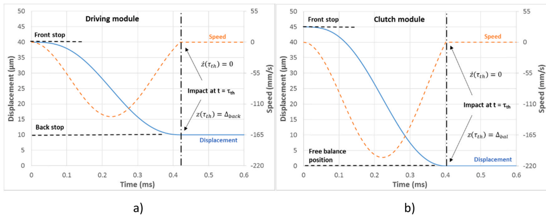
Fig. 11. Evolution of the displacement and the speed in the case of the driving module (a) and the clutch module (b) for the optimal voltage fall time.
