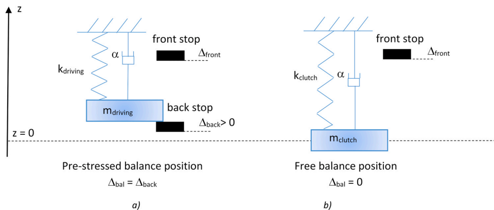
Fig. 10. Schematic representation at the end of the “elastic restored” motion (a) Final position of the driving module against the back stop at \Delta_{back} = 10 \mu\text{m} (b) Final position of the clutch module at the balance position at \Delta_{bal} = 0 .
