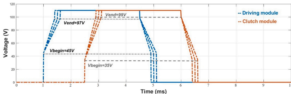
Fig. 8. New chronogram with shaped command signals for the two-module comb-drive actuator.
