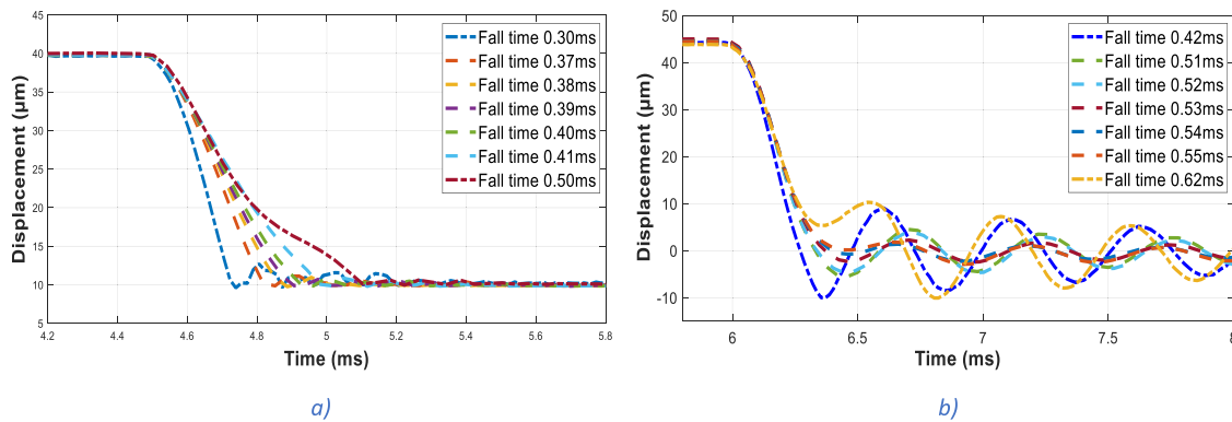
Fig. 14. Influence of the voltage fall time in the “elastic restored” motion in the case of a) the driving module and b) the clutch module.
