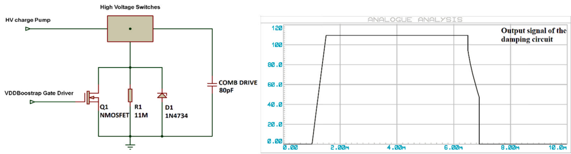
Fig. 17. Damping circuit design and its output signal.
