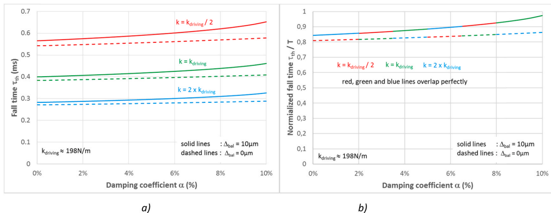
Fig. 12. Evolution of the fall time \tau_{th} as a function of the damping coefficient a) and corresponding evolution of the normalized fall time \tau_{th}/T b) based on nominal parameters of the driving module.
