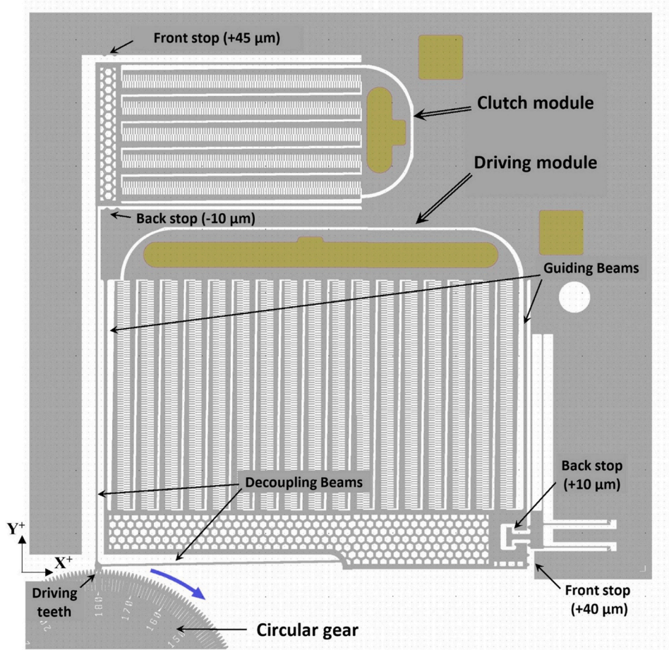
Fig. 1. Layout of the two-module comb-drive actuator with the circular gear to be driven.
