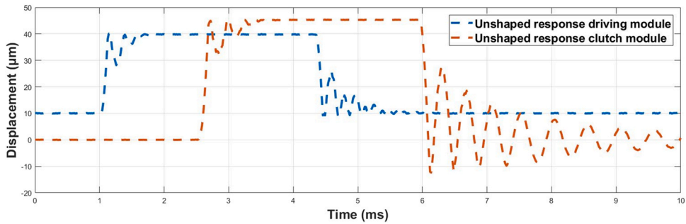
Fig. 5. Mechanical responses of the two modules according to the unshaped command signals.
