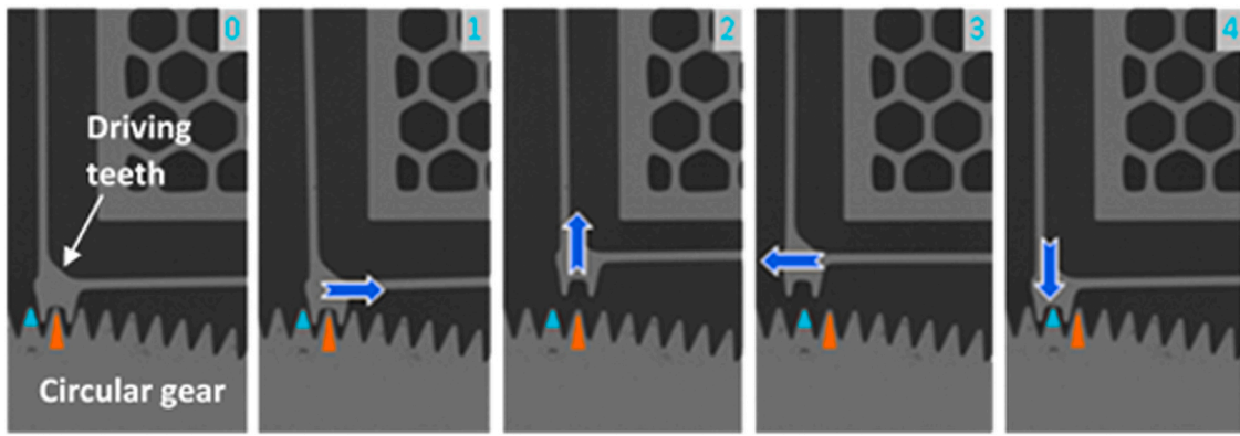
Fig. 2. Chronological sequence to drive a circular gear in the clockwise direction.
