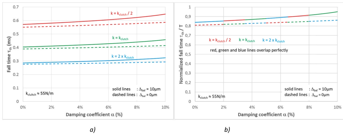
Fig. 13. Evolution of the fall time \tau_{th} as a function of the damping coefficient a) and corresponding evolution of the normalized fall time \tau_{th}/T b) based on nominal parameters of the clutch module.
