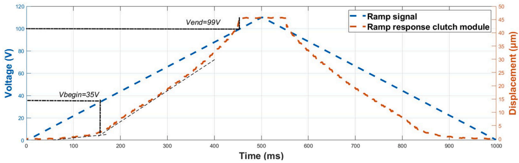
Fig. 7. Electromechanical characterization of the clutch module displacement as function of voltages.
