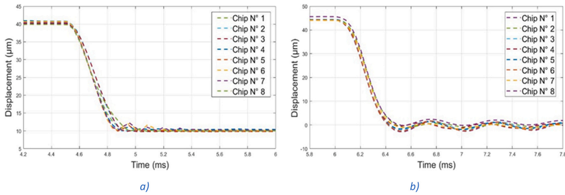
Fig. 15. Dynamic behavior of a set of 8 MEMS chips in the “elastic restored” motion in the case of a) the driving module and b) the clutch module.
