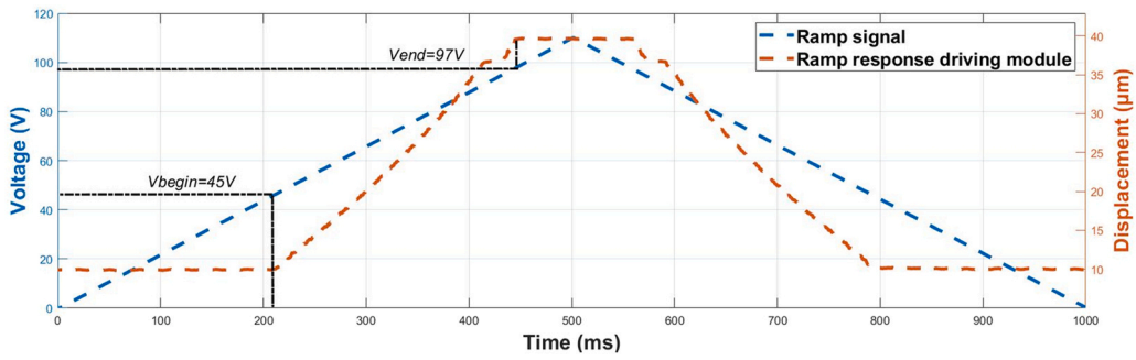
Fig. 6. Electromechanical characterization of the driving module displacement as function of voltages.
