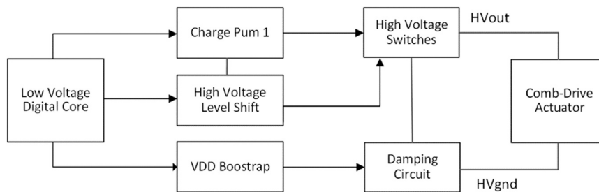
Fig. 16. Block diagram of the MEMS control circuit.
