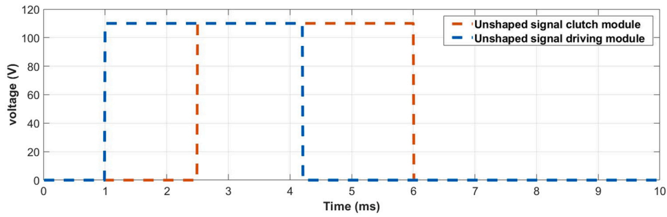
Fig. 4. Chronogram of the unshaped signals for driving the two-module comb-drive actuator.
