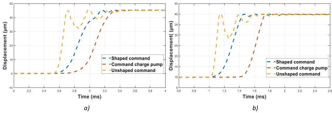
Fig. 9. Resulting motion from a typical electrical signal delivered by an integrated charge pump: a) Displacement of the driving module, b) Displacement of the clutch module.
