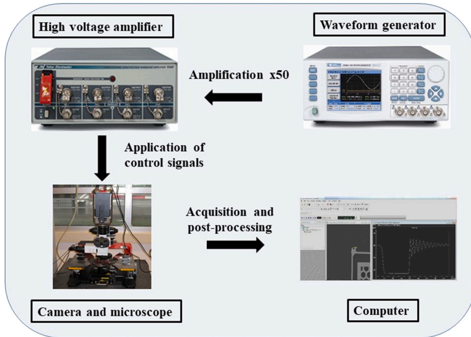
Fig. 3. Instrumentation chain for the displacement tracking of the driving and clutch modules.
