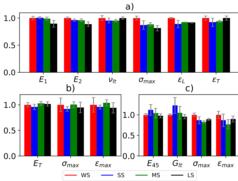
Fig. 7 Effects of the embedding of inserts on the mechanical properties in traction for a) [0] 20 laminates, b) [90] 20 laminates and c) [45] 20 laminates
