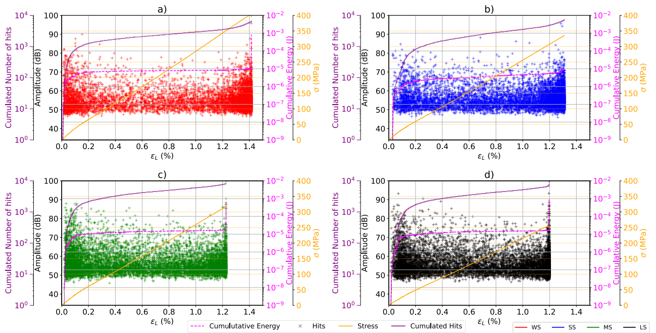
Fig. 9 AE Hits, cumulative energy and cumulative number of hits as a function of tensile strain for [0]_{20} laminates. a) pristine laminate (WS), b) embedded with small sensor (SS), c) embedded with medium sensor (MS) and d) embedded with large sensor (LS)
