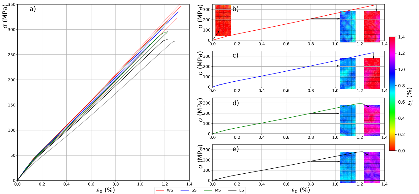
Fig. 5 Tensile stress-strain curves of pristine and embedded flax-epoxy fibres oriented laminates. a) 0^\circ ( [0]_{20} samples) for all tested samples' sensor size. Representative tensile stress-strain curve in 0^\circ direction for samples: b) Without sensor (WS), c) with Small Insert (SS), d) with Medium Insert (MS) and e) with Large Insert (LS) with longitudinal strain field obtained by DIC at 200MPa and just before failure.
