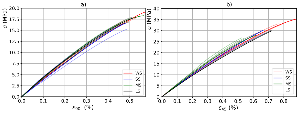
Fig. 6 Tensile stress-strain curves of pristine and embedded flax-epoxy laminates. Results for a) 90°([90] 20 samples) and b) 45°([45] 20 samples)
