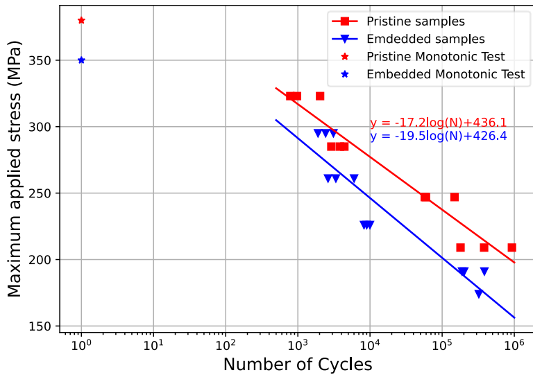
Fig. 12 S-N curve for embedded and pristine samples obtained for tensile-tensile fatigue tests.
