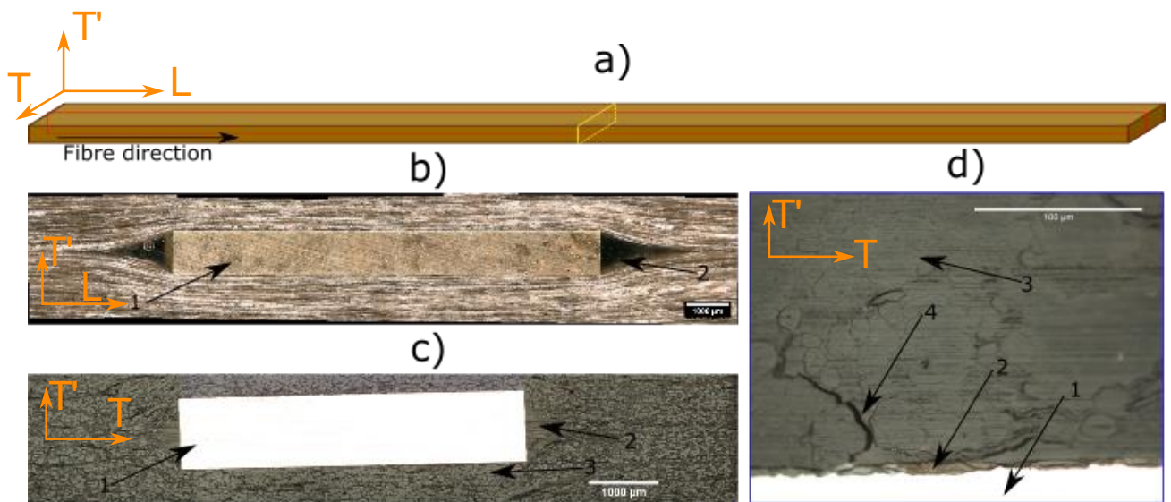
Fig. 3 Cross section of samples with embedded LS inserts. a) 3D representation of the samples and the material planes with ( LT' ) plane in red and ( TT' ) plane in yellow. b) ( LT' ) cross section c) ( TT' ) cross section d) microcracks observed in the ( TT' ) cross-section. 1: dummy sensor, 2: matrix rich region, 3: fibre bundles, 4: microcracks
