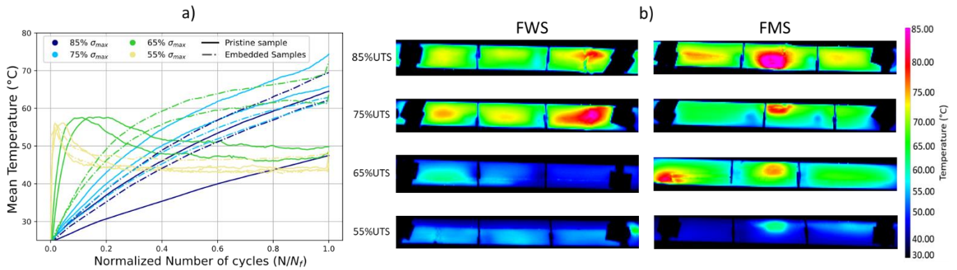
Fig. 13 a) Mean surface temperature and b) Surface temperature field obtained by infrared thermography during tensile-tensile fatigue testing for pristine (FWS) and insert embedded in samples (FMS) at 85%, 75%, 65% and 55% of the ultimate tensile stress (UTS)
