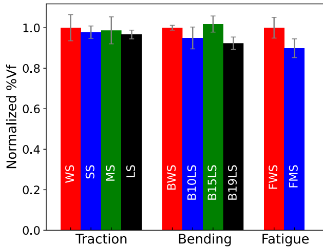
Fig. 4 Influence of the insert embedding on the fibre volume fraction. Results are normalised using the average value of the fibre volume fraction of the pristine samples (the bars represent the mean values and error bars the standard deviation).
