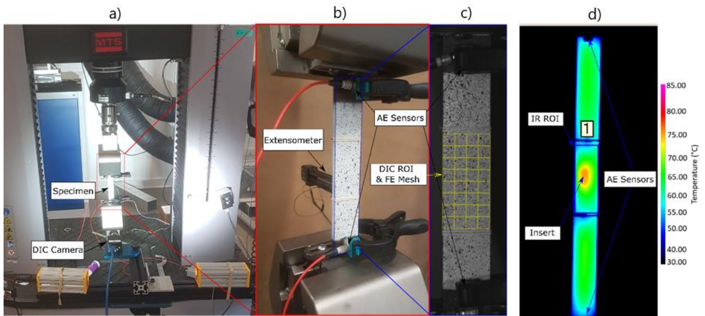
Fig. 2 a) Experimental set-up for the monotonic tensile tests with b) acoustic emission and DIC speckle and c) superposed finite element mesh. d) Thermal variation observed at the surface of the specimens by IR camera during fatigue loading
