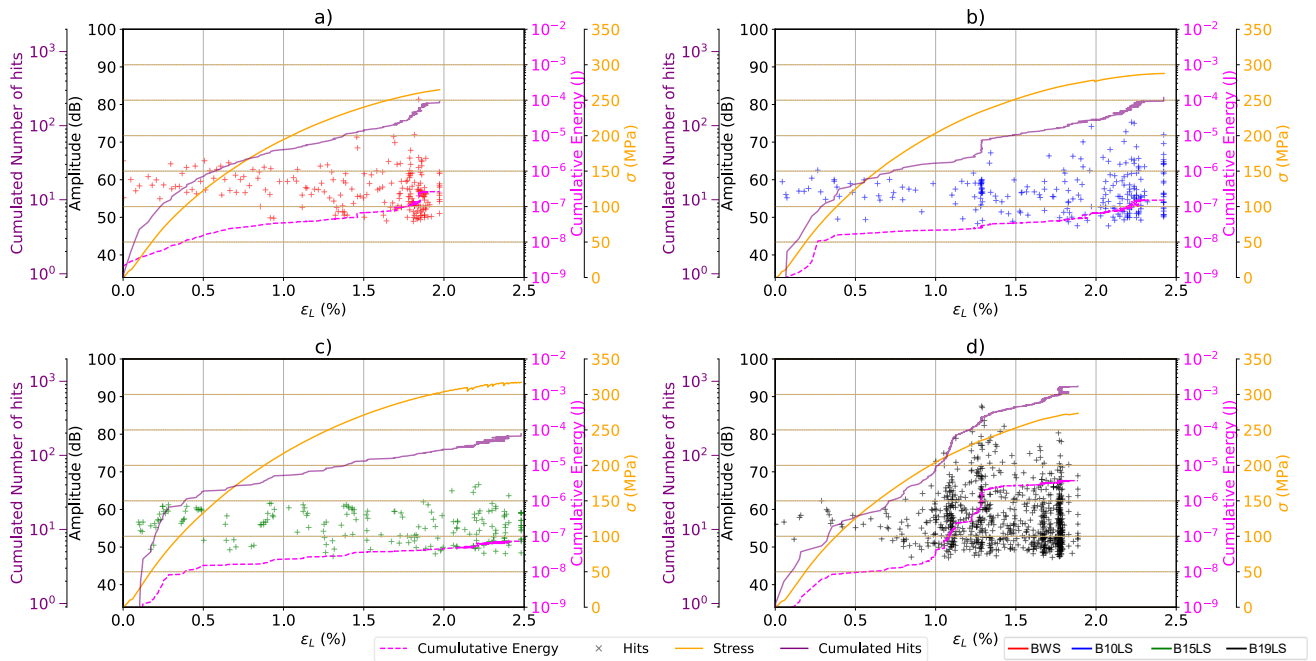
Fig. 11 Monotonic bending AE data (amplitude, cumulative energy, cumulated hits) as a function of maximum bending strain. a) BWS b) B10LS c) B15LS d) B19LS
