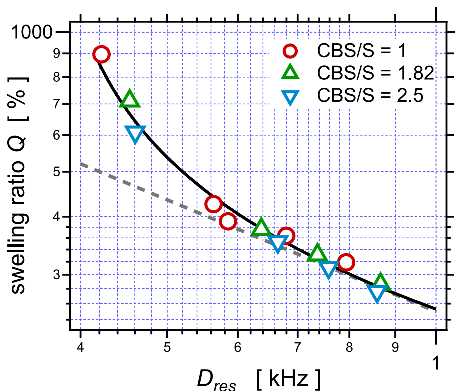
Figure 6. The equilibrium swelling ratio Q (in vol%) as a function of the NMR parameter D_{res} for the series of samples with different amounts of sulfur and different sulfur/accelerator ratios. The plain curve is a fit of the full set of data with the Flory–Rehner equation (Equation (11)), taking the assumption of phantom network, as described in the text.
