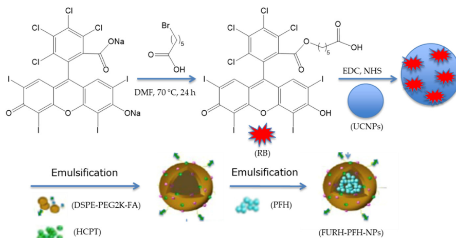
Figure 16. Preparation of FURH-PFH-NPs. Adapted from Wang et al. [39].
