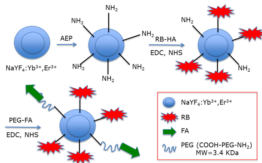
Figure 1. Covalent coupling of \text{NaYF}_4:\text{Yb}^{3+} and \text{Er}^{3+} UCNPs with RB and FA. Adapted from Liu et al. [20].
