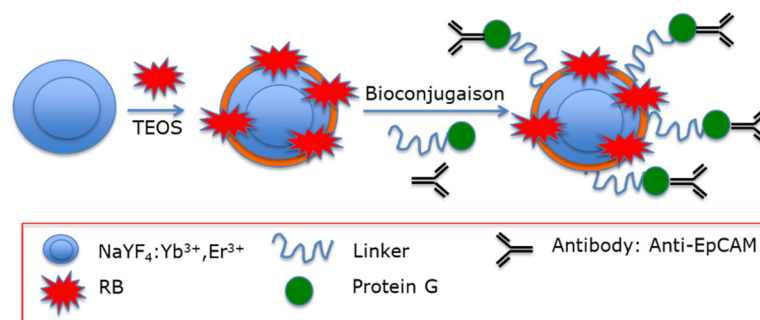
Figure 9. Covalent coupling of RB and antibody through a bifunctional fusion protein G. Adapted from Liang et al. [26].
