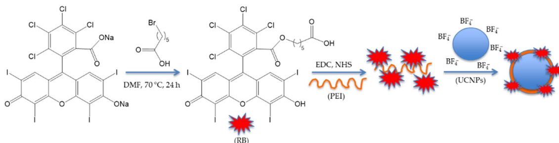
Figure 6. Covalent coupling of RB onto Er@Nd UCNP. Adapted from Li et al. [25].
