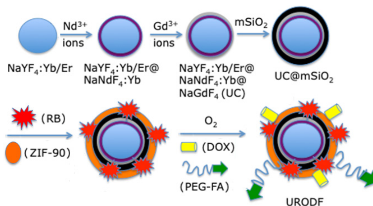
Figure 13. Preparation of URODF NPs. Adapted from Xie et al. [34].
