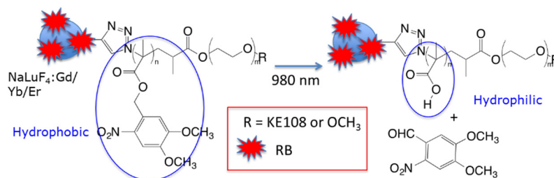
Figure 11. Illustration of NIR-triggered hydrophobic-to-hydrophilic transition leading to the release of hydrophobic drug. Adapted from Chen et al. [28].
