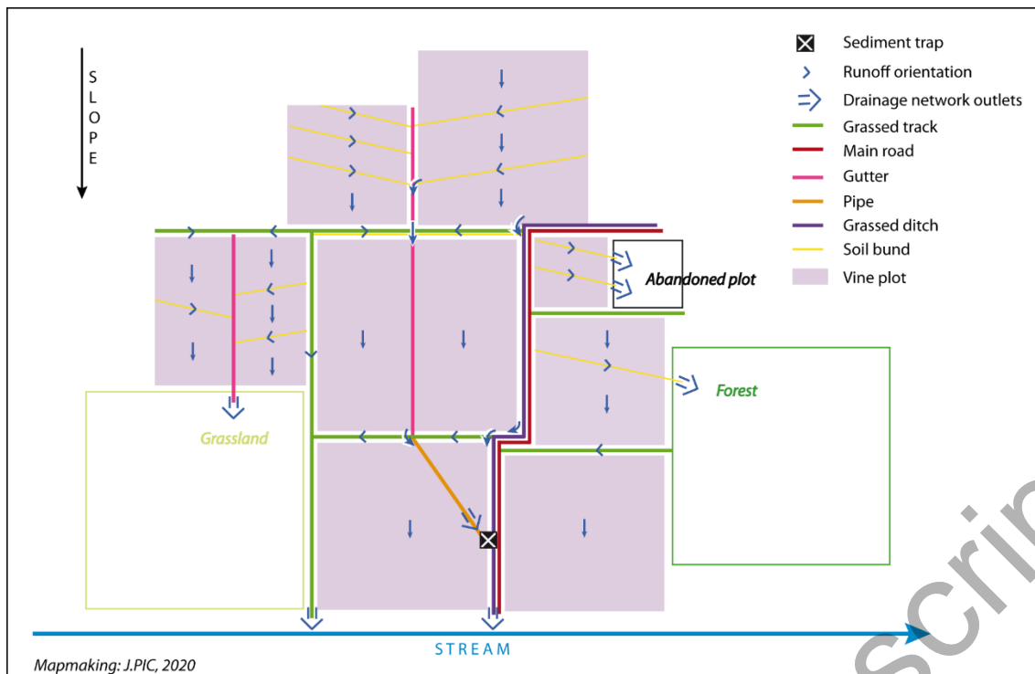
Figure 9. Sketch of the influence of linear infrastructure on runoff and associated sediment pathways
