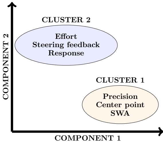
Fig. 1. System's dimensions reduction with PCA
