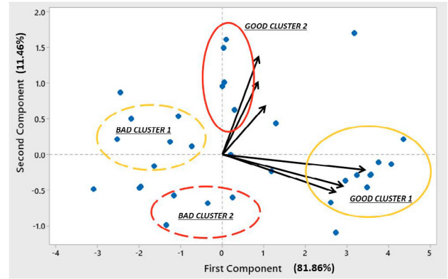
Fig. 2. Redistribution of data points according to the 2 main components
