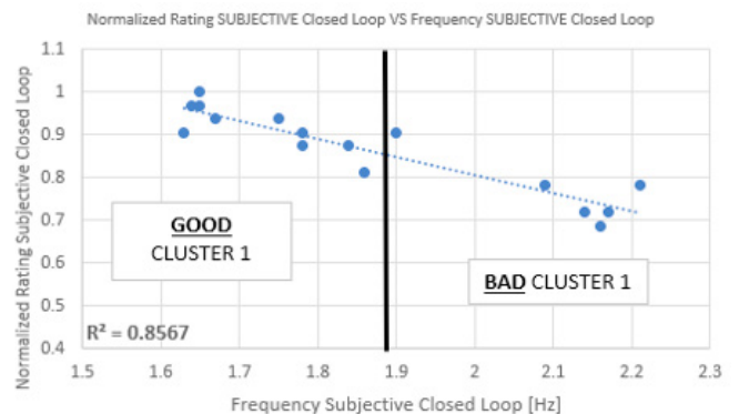
Fig. 8. Correlation between the Normalized Rating for the subjective closed loop and the frequency chosen by the driver during the subjective closed loop
