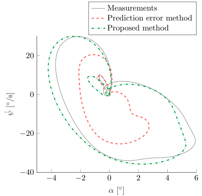
Fig. 7. Trajectories in the state-space
