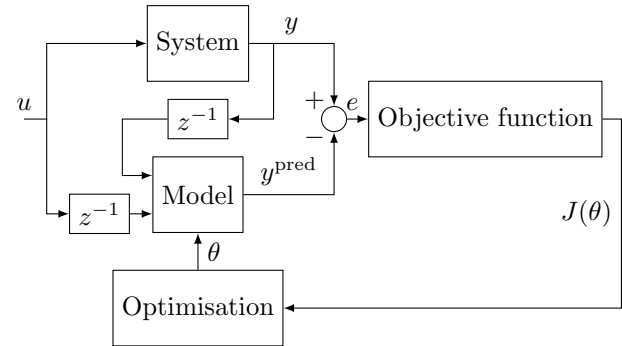
Fig. 1. Scheme of the prediction error method
