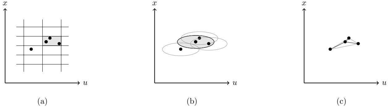
Fig. 3. Illustration of the different weighting techniques: (a) grid in the state and input space, (b) ellipses around the samples, (c) distances between samples. Samples are represented as •.
