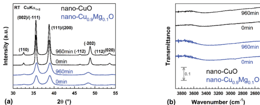
Fig. 5 XRPD patterns (a) and IR transmission spectra (b) collected ex situ and at room temperature (RT) on the nanometer-sized particles of CuO and Cu_{0.9}Mg_{0.1}O before and after 960 min of immersion in liquid water.
