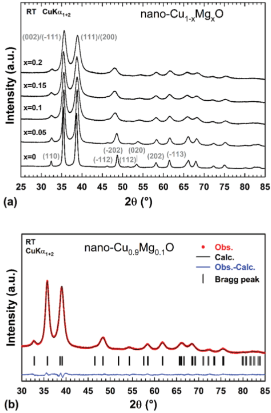
Fig. 1 (a) XRPD patterns recorded under an ambient air atmosphere (60% RH) and room temperature (RT) for nanometer-sized \text{Cu}_{1-x}\text{Mg}_x\text{O} particles for different magnesium contents x . The (hkl) values of the first crystal planes are given. (b) Comparison of the observed diffraction pattern of nanometer-sized \text{Cu}_{0.9}\text{Mg}_{0.1}\text{O} ( x = 0.1 ) particles (red dots) with the pattern calculated by the integral breadth method (black line). The blue curve corresponds to the difference between observed and calculated patterns. Vertical markers give Bragg peak positions for the CuO-type phase (space group C2/c (no. 15)).
