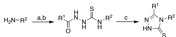
Scheme 1. Synthesis of 4-phenylalkyl-1,2,4-triazole-3-thione derivatives. Reagents and conditions: (a) DPT, DMF, sealed tube, 55 °C, 3h; (b) R^1 -CONHNH 2 , DMF, 55 °C, 3h; (c) aqueous KOH or NaHCO 3 , 100 °C, 3h.
