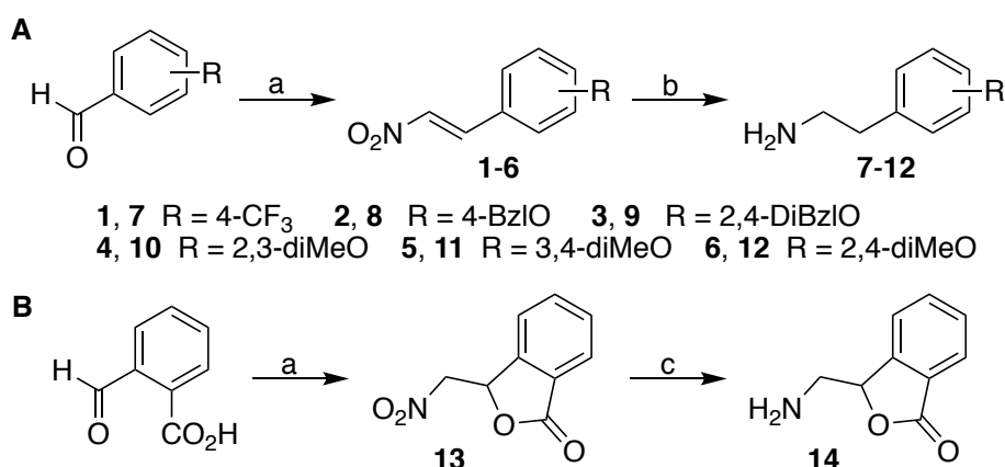
Scheme 2. Synthesis of the phenethylamines R^2 -NH 2 7-12 (A) and 14 (B). Reagents and conditions: (a) Nitromethane, NH 4 AcO, AcOH, 120 °C, 15h; (b) LiAlH 4 , THF, 80 °C, 15h; (c) AcOH, HCl, Zn powder, 16h, r.t.
