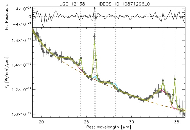
Figure 7. Example of a fit to the 19\text{--}35.5\ \mu\text{m} spectrum of an IDEOS source. The observed spectrum is shown in black, the fit to the data in green. The local continuum is shown in pink, and the continuum corrected for crystalline silicate emission in brown. Upper limits for undetected lines are shown in cyan. Vertical lines denote commonly detected features: 24.32\ \mu\text{m} [Ne V], 25.89\ \mu\text{m} [O IV], 25.99\ \mu\text{m} [Fe II], 28.22\ \mu\text{m} \text{H}_2 S(0), 33.48\ \mu\text{m} [S III], and 34.82\ \mu\text{m} [Si II].
