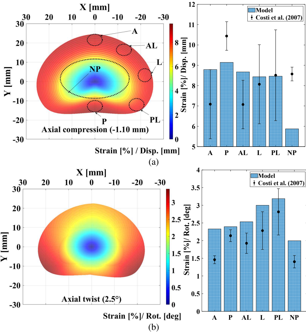
Figure 9. Predicted normalized radial strains (%/mm) in a disc (a) compressed at 1.1 mm and (b) twisted at 2.5°. The comparison to Costi et al. [52] data is performed for different regions in which the local strains are averaged (A: Anterior, P: Posterior, AL: Anterior-Lateral, L: Lateral, PL: Posterior-Lateral, NP: nucleus pulposus).
