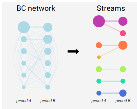
Fig. 1: Matching clusters from successive time periods. We start with the BC network built from clusters of publications detected independently in periods A and B. For each cluster a of period A and cluster b of period B, we compute the modularity change \delta Q_{ab} obtained by grouping these two clusters in the 2-periods BC network. The ‘successor’ of cluster a is defined as the cluster b from period B maximizing this quantity and the ‘predecessor’ of cluster b is defined as the cluster a from period B maximizing this quantity. In the stream visualisation, ‘paired’ clusters (successor / predecessor of each other) are represented on the same y-position, and we only show the BC links between successors or predecessors, which highlight dynamical events such as merge and splits. In these figures, the size of the nodes are proportional to the number of publications in the corresponding clusters and the thickness of the links represent the average weights of the BC links between publications from two clusters.
