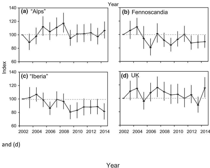
FIGURE 3 Regional mountain bird indicators during 2002–2014 from (a) “Alps”, (b) Fennoscandia, (c) “Iberia”
