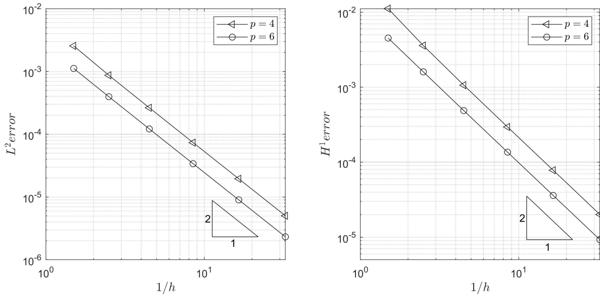
Figure 3: The error plots in the L^2 norm (left) and in the H^1 norm (right) as a function of 1/h for the example of Section 6.2 with a solution of limited regularity using p = 4, 6 , \Delta t = 10^{-3} , q = 2 , and a discretization with an odd number of elements in the x direction.
