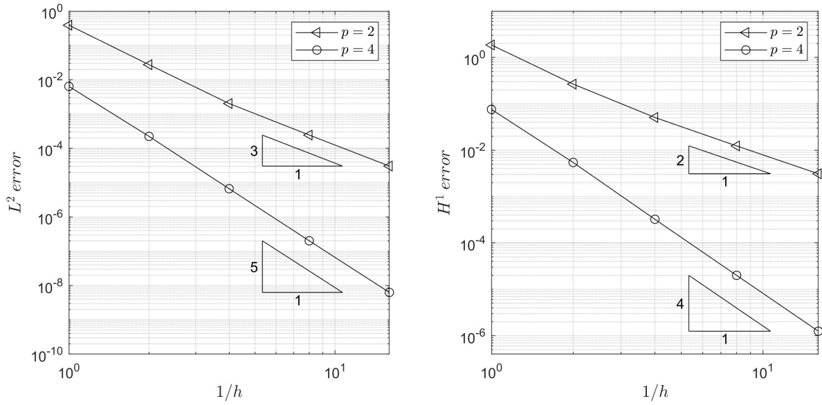
Figure 1: Convergence of the error in the L^2 norm (left) and in the H^1 norm (right) as a function of 1/h for the example of Section 6.1 with a regular solution using p = 2, 4 and \Delta t = 10^{-4} .
