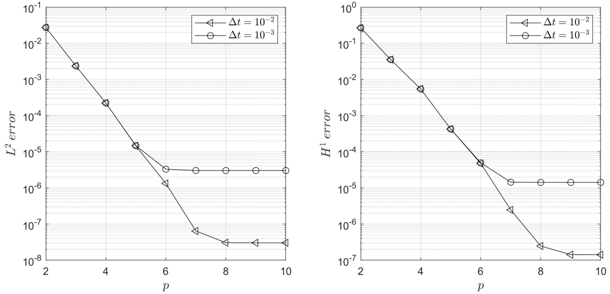
Figure 2: Convergence of the error in the L^2 norm (left) and in the H^1 norm (right) as a function of p for the example of Section 6.1 with a regular solution using \Delta t = 10^{-2} and \Delta t = 10^{-3} but a fixed h = 1/2 .
