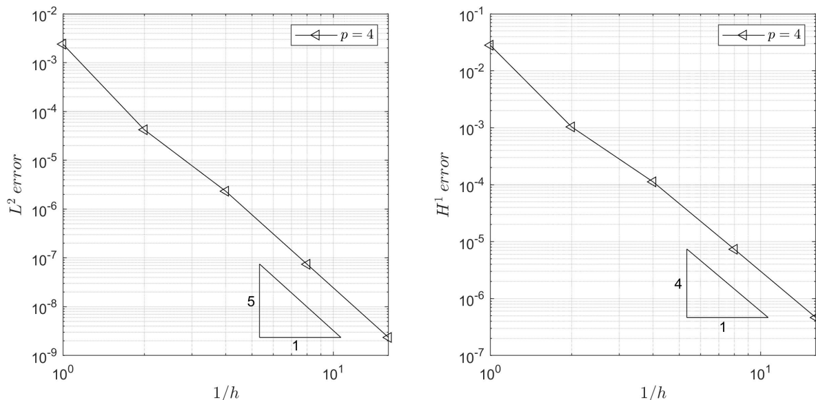
Figure 6: The error plots in the L^2 norm (left) and in the H^1 norm (right) as a function of 1/h for the example of Section 6.2 with a solution of limited regularity using p = 4 , \Delta t = 10^{-3} , q = 2 and a discretization with an even number of elements in the x direction.
