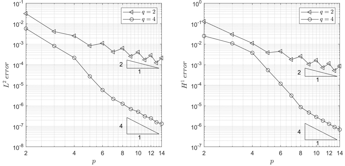
Figure 5: The error plots in the L^2 norm (left) and in the H^1 norm (right) as a function of p for the example of Section 6.2 with a solution of limited regularity using q = 2, 4 , \Delta t = 10^{-3} , and h = 2/3 (i.e. the mesh consists of three elements in the x direction).
