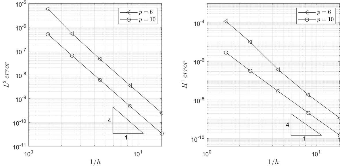
Figure 4: The error plots in the L^2 norm (left) and in the H^1 norm (right) as a function of 1/h for the example of Section 6.2 with a solution of limited regularity using p = 6, 10 , \Delta t = 10^{-3} , q = 4 , and a discretization with an odd number of elements in the x direction.
