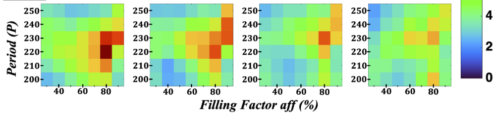
Fig. 4. Enhancement of the integrated absorbance with backbone made of holes (left) and pillars (right) structure, in spectral range [340–375 nm], for t = 210 nm for both holes and pillars.
