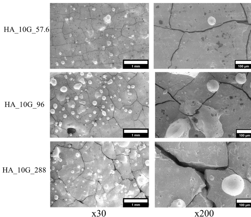
Fig. 10. SEM analyses of laser-induced circular patterns produced with same powder feedstock blend (HA_10G) at different E_d : 288 J\ cm^{-3} , 96 J\ cm^{-3} , 57.6 J\ cm^{-3} . Analyses of sample HA_10G_96 are repeated here for better comparison.
