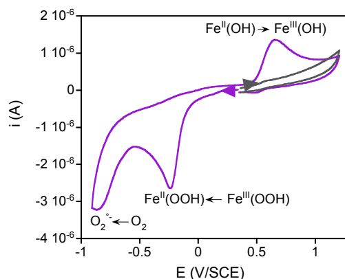
Figure 2. Cyclic Voltammogram of [\text{Fe}^{\text{III}}(\text{OOH})(\text{L}_5^2)](\text{PF}_6)_2 (1 mM) in PrCN + 0.2 M TBAPF 6 at -70^\circ\text{C} , 0.1 \text{ V}\cdot\text{s}^{-1} . The arrows indicate the initial direction of the scan.
