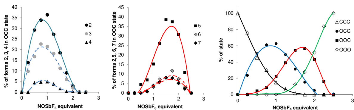
Figure 8. Quantification of the forms in OCC and OOC states and of the 4 different states of compound 7b (1 mM) in ACN upon addition of NOSbF 6 aliquots.
