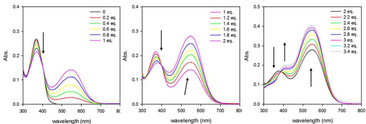
Figure 7. Variation of the UV-Visible spectrum of 7b ( 9 \times 10^{-6} M) in ACN upon the addition of \text{NOSbF}_6 aliquots.
