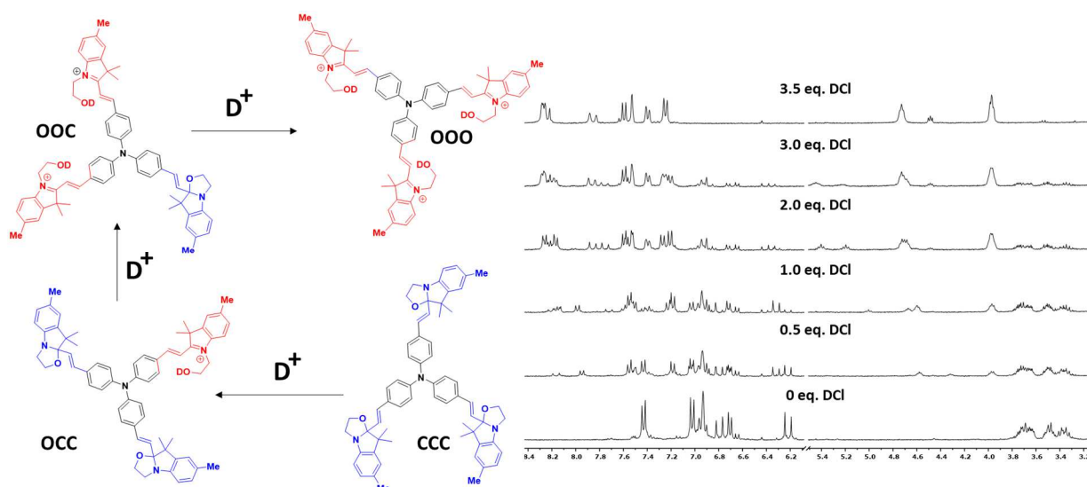
Figure 3. Variation of the ^1\text{H} NMR spectra of compound 5b (4.62mM) in ACN solution upon the addition of DCl aliquots at 20°C translating the successive formation of OCC , OOC and OOO states.
