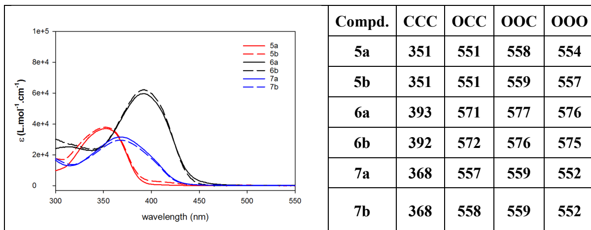
Figure 1. UV visible spectra of compounds 5-7 under their fully closed states, CCC, and evolution of their maximum absorption wavelength ( \lambda_{\max} in nm) under acid stimulation as function of the open (O) or closed (C) status of the three BOX units.
