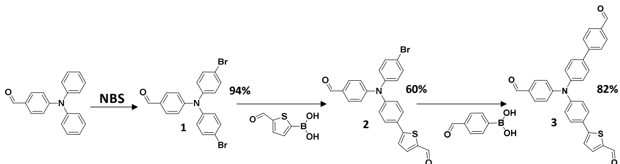
Scheme 3. Synthesis of the tricarboxaldehyde amine involving 3 different linkers: a phenyl (Ph), a phenylthiophene (PhTh) and a biphenyl (PhPh).
