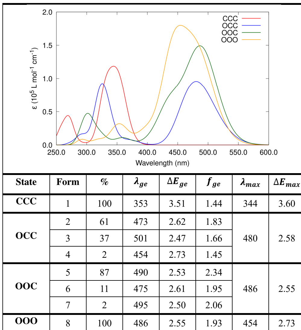
Vertical excitation wavelengths ( \lambda_{ge} , nm), vertical excitation energies ( \Delta E_{ge} , eV) and oscillator strengths ( f_{ge} ) of the first excited state. The maximal excitation wavelengths ( \lambda_{max} , nm) and energy ( \Delta E_{max} , eV) of the different states, accounting for their relative proportions, are also reported. The averages are weighted using the populations of conformers at 298.15 K as calculated at the \omega B97X-D/6-311-G(d)/IEF-PCM (ACN) level of theory.
