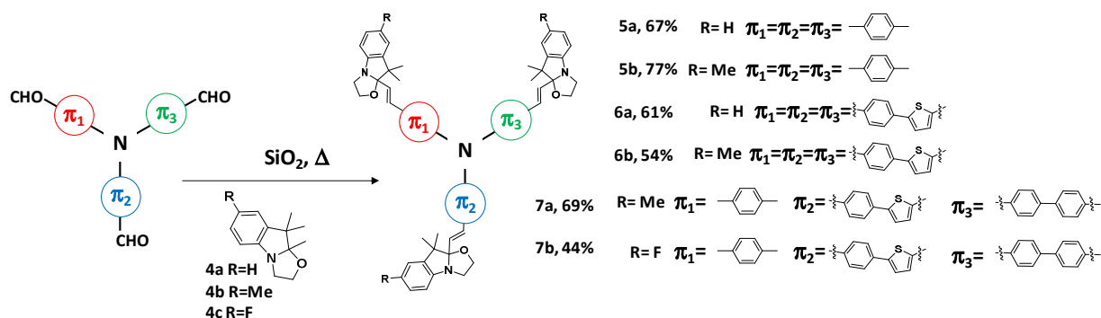
Scheme 3. Synthesis of the 4 symmetrical and 2 unsymmetrical triBOX derivatives by silica mediated procedure from the corresponding tris-carboxaldehyde amine.
