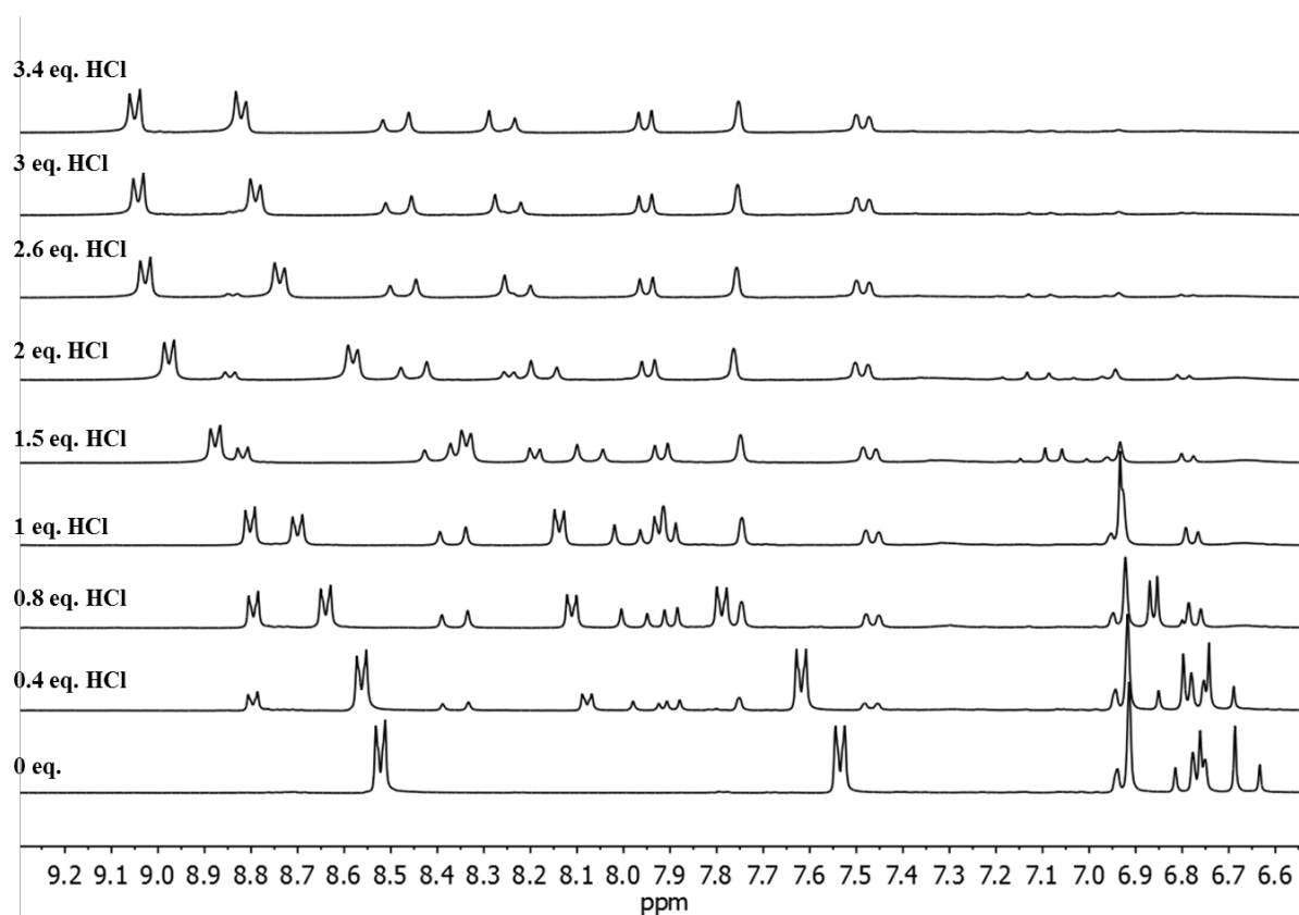
Figure 3. ^1\text{H} NMR spectra upon titration of 4b (14 mM) by HCl in \text{DMSO-d}_6 at 20^\circ\text{C} up to 3.4 equivalents
