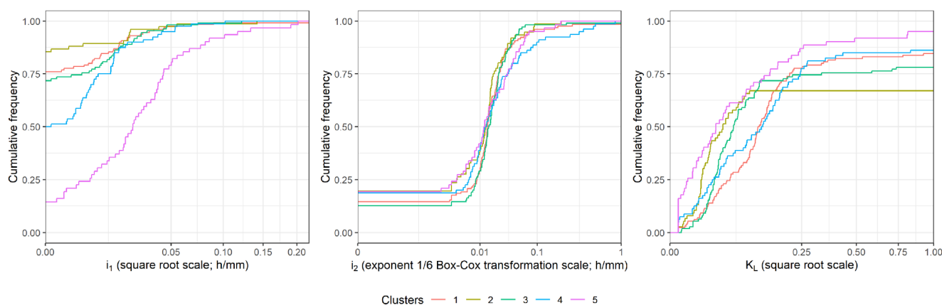
FIGURE 12 Distributions of the additional M3-Pr-B free parameters for five groups of catchments
