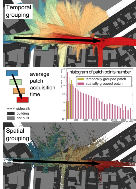
Figure 14: Temporal (top) and spatial (bottom) grouping on velodyn terrestrial Lidar data, with histogram of number of points per patch.
