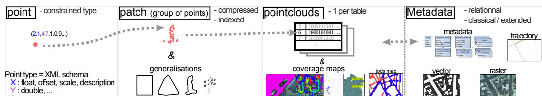
Figure 2: PgPointCloud storage illustration. Point attributes are described by an XML schema. Points are grouped in patches, indexed and compressed, which may have several generalisations. A point cloud is stored in a table, with one patch per row, along with other tables generalising the point cloud (like coverage map). The PCS also stores meta-data (date, place) in a relational way, extended meta-data like trajectories, and possibly other GIS data like vector and rasters.
