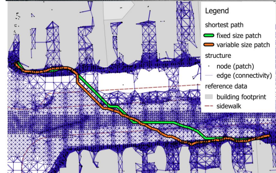
Figure 22: Two views of shortest path on regular (yellow) and varying (orange) size patches.~ 100ms
