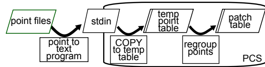
Figure 6: Conceptual schema for parallel loading.
