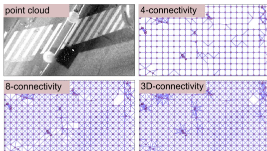
Figure 21: Example of possible connectivity by connecting patch centres that are closer (3D distance) than a threshold (1.4, 1.5, 1.9 metres).
