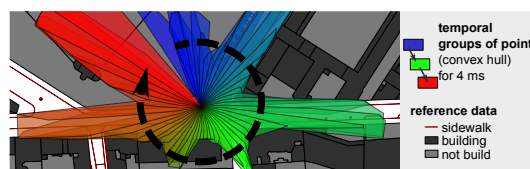
Figure 3: Rotating Lidar (Velodyn) with strong temporal dependency (200 ms acquisition).
