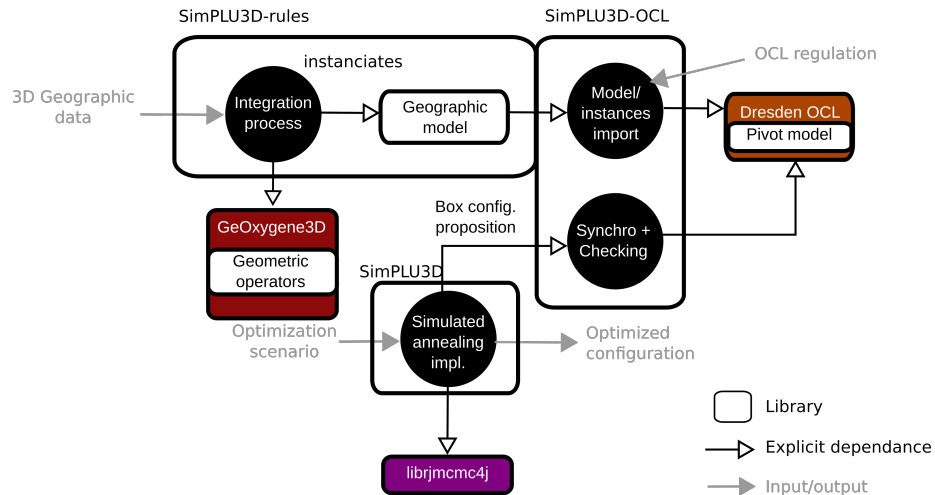
Figure 7: Architecture of the implemented prototype.
