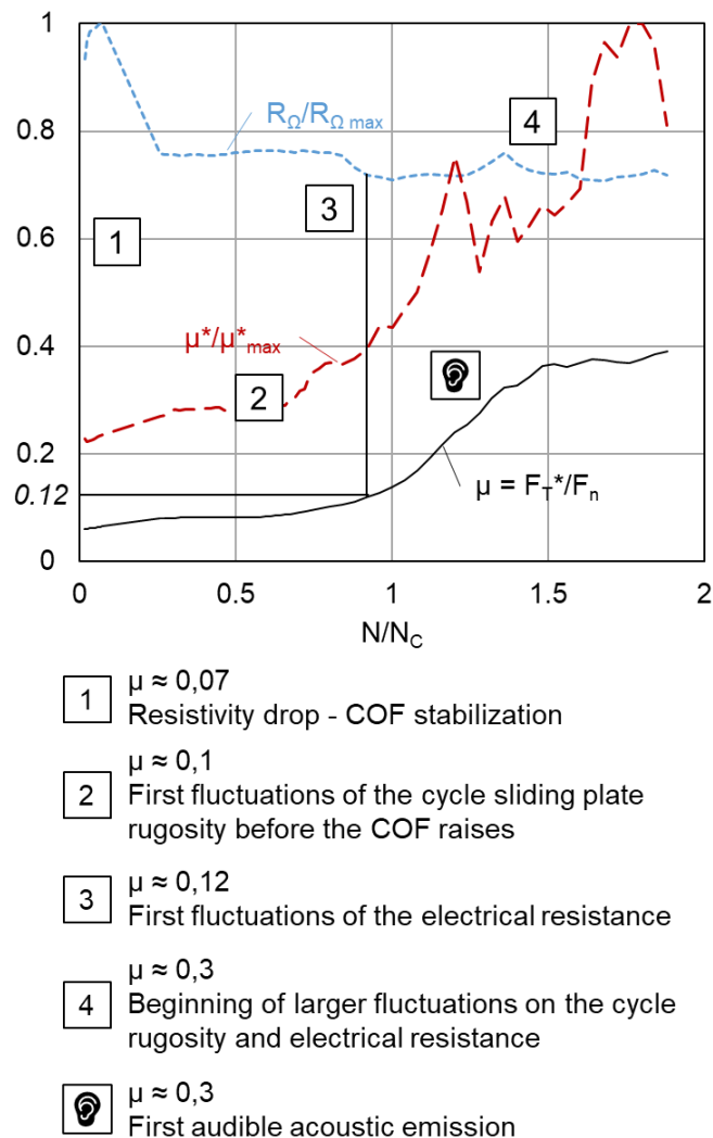
Figure 10 Evolution of the COF, \mu^* (normalized by \mu^*_{\max} ) and R_\Omega (normalized by R_{\Omega \max} ) for a typical sliding test F_n = 40 kN, f = 0.2 Hz, \theta^* = \pm 25^\circ , D = \pm 15 mm)
