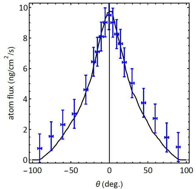
Figure 8: Comparison between the experimental differential mass flux measured in the micro-scale and the Monte-Carlo simulation at T=898K .
