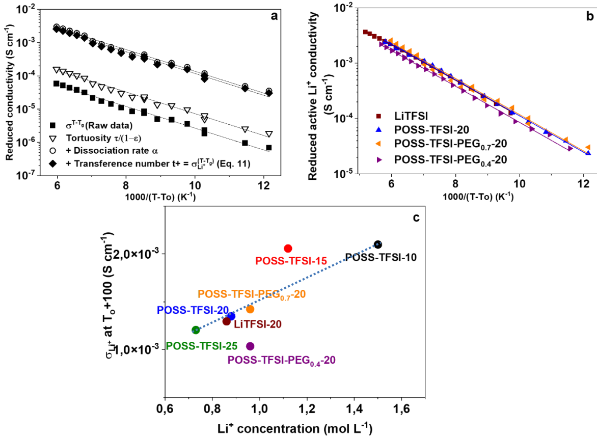
Figure 8. a) Evolution of \text{Li}^+ reduced conductivity of POSS-TFSI-PEG 0.7 -20 corrected by the tortuosity, dissociation rate, and transference number t^+ thanks to eq. 11 (and 12) ; b) The “true” reduced \text{Li}^+ conductivity compared for the different TEG based electrolytes calculated according to Equation 11, using parameters measured experimentally and listed in Table 2 and Table 4; c) “True” \text{Li}^+ conductivity at the same distance to the glass transition temperature ( T_0+100 ) as a function of \text{Li}^+ concentration.
