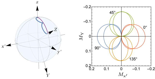
Figure A.1: Left: The rotating ( x', y', z ) and doubly-rotating ( x'', Y, Z ) frames with simulations starting from unit equilibrium magnetization for a CP field (thin purple line) and linear field (thick blue line) with B_1 = B_\omega/\nu_\pi (here \nu_\pi = 3 ), \delta B = 0 , \phi_r = 0^\circ , and \phi_s = \phi_d = 90^\circ . The trajectories are shown for a single rf period. The terminus of the trajectory for the linear field has a noticeable non-zero M_{x''} component. Right: Components of the transverse magnetization in the doubly-rotating frame shown for simulations with \delta B_p(\phi_s) of Eqs. 8 and 9 for a variety of start phases ( \phi_s = \phi_d , indicated on the graph) for a single period of a linear rf field. All other parameters are the same as above. Under these conditions, M_{x''} \approx M_Y \approx 0 every half-period from the start of the pulse. Deviations from perfect nullification (not visible at this scale for this example) can be eliminated by a small change in B_1 and a higher order correction in \delta B_p , as discussed in Sec. 3.2.
