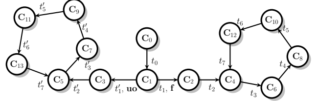
Fig. 2. Part of a SCG exhibit the transition sequences of two paths and the visited classes associated
