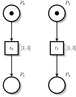
Fig. 1. LTPN illustrating the constraints imposed by parallelism in a system
