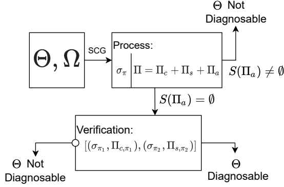
Fig. 3. Synthetic diagram for checking diagnosability of a timed fault \Omega on a system \Theta
