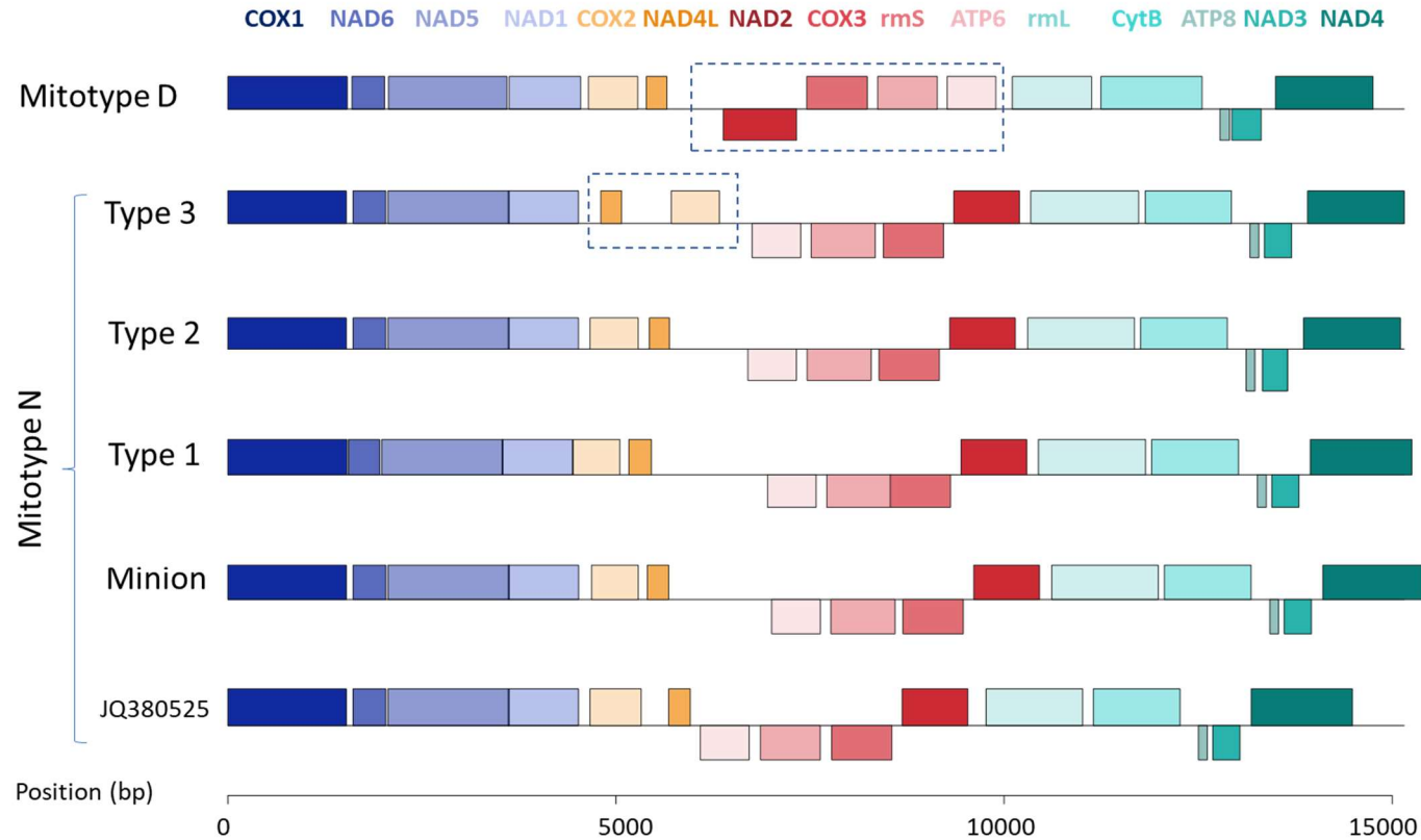
Figure S1. Structural variants in the assembled mitogenomes of D and N individuals of P. acuta . Related to Figure 1. Gene orders are displayed for 20 reassembled mtDNA sequences from transcriptomes of the Lyon population, falling into four structural variants: one for the D mitotype (10 individuals) and three for the N mitotype (4, 3 and 3 individuals of type 1, 2 and 3 respectively). We also represent the mtDNA of another N individual collected in a natural population near Lyon (see Methods) obtained from a MinION long-fragment sequencer (“Minion”) – its similarity with other N individuals rules out any strong bias specific to transcriptome-based assembly. The JQ380525 sample (referred by its Genbank accession number) is isolate A from New Mexico (USA S1 ) and is also of mitotype N. For easier reading, the mitogenomes are represented in linear form, tRNA genes are omitted, boxes are represented above or below the line depending on whether the coding sequence is on the “+” or “-” strand, and zones with changes in gene order, compared to the JQ380525 reference, are framed in a blue dotted line. The details of annotations are represented in Table S1.
