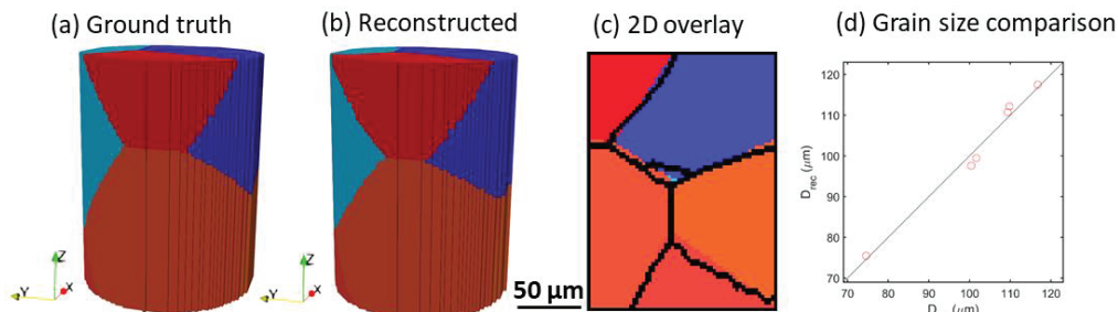
Figure 2. Comparison of reconstructed grain structure by LabDCT with the ground truth input. (a) Ground truth input and (b) reconstructed structures visualized in 3D; (c) overlay of grain boundaries in the reconstructed grain map onto the corresponding XZ slice of the ground truth; (d) grain size comparison between the ground truth and the LabDCT reconstruction. Grains are colored in IPF-Z direction. Voxel size is 2.5 \mu\text{m} .
