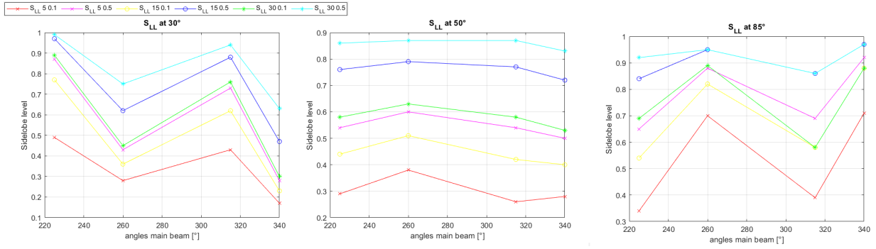
Fig. 4. S_{LL} at 30°, 50° and 85° angle of incidence of the cluster of scatterers.
