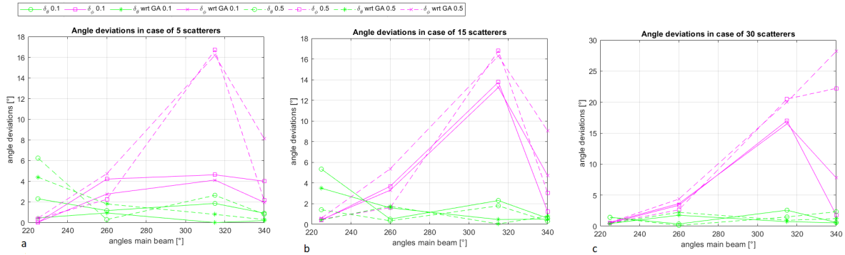
Fig. 5. Angle deviations with 30° angle of incidence of the cluster of scatterers.
