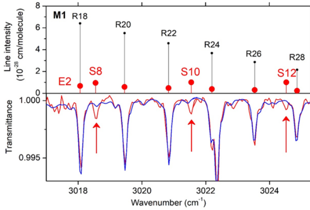
FIG. 2. Comparison of the ACS MIR transmission spectra of the atmosphere of Mars [19] near 3020\text{ cm}^{-1} with calculated line lists of the M1 and E2 \nu_2 + \nu_3 bands of ^{12}\text{C}^{16}\text{O}_2 . Upper panel: The presently calculated E2 transitions with ab initio intensities (red stems) are superimposed to the M1 transitions with intensities measured in [19] (black stems). Lower panel: ACS MIR spectrum (red line) with a best-fit synthetic model containing the contributions of the E1 bands of \text{CO}_2 and \text{H}_2\text{O} based on HITRAN 2016 database and of the M1 lines identified in [19]. The assignments of the newly detected S8–S12 E2 transitions are marked with red arrows.
