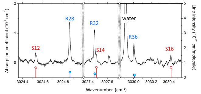
FIG. 3. Comparison of the laboratory spectrum of \text{CO}_2 at 60 mbar recorded by OFCEAS [23] with the calculated E2 line list of ^{12}\text{C}^{16}\text{O}_2 in three spectral intervals of the E2 \nu_2 + \nu_3 band. The R - and S -band transitions are plotted with blue and red stems, respectively. The S12, S14 and S16 E2 lines are apparent. The line intensities of the R28, R32 and R36 transitions is mostly due to the M1 transitions.
