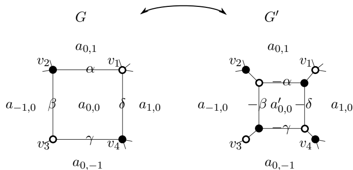
Figure 8: The “urban renewal” transformation; the greek letters represent the Kasteleyn orientation, and non-indexed edges on the right-hand side are given orientation 1, i.e. , from white to black.
