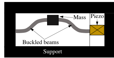
Figure 8. Example of bistable PEH where the piezoelectric voltage acts nonlinearly on the harvester dynamics. The piezoelectric energy harvester is a buckled beam structure. The piezoelectric material is fixed between one of the buckled beam and the support.
