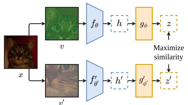
FIGURE 1 – Common base shared by recent methods. The input image x is augmented in two ways to give the views v and v' . These views are then passed through an encoder to give respectively the representations h and h' , which are then passed in a projection head that outputs respectively the embeddings z and z' on which the loss is applied.
